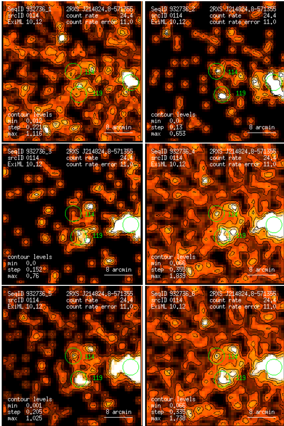
Figure 114: RASS 932736: detection 0114: band rate images, Gaussian filter: (1) PSPC channels 11 – 41, (2) 52 – 90, (3) 91 – 201, (4) 11 – 235, (5) 52 – 201, (6) 11 – 201. Broad band rates in counts/ks. Band rate contour levels in counts/ks/arcmin 2 .
