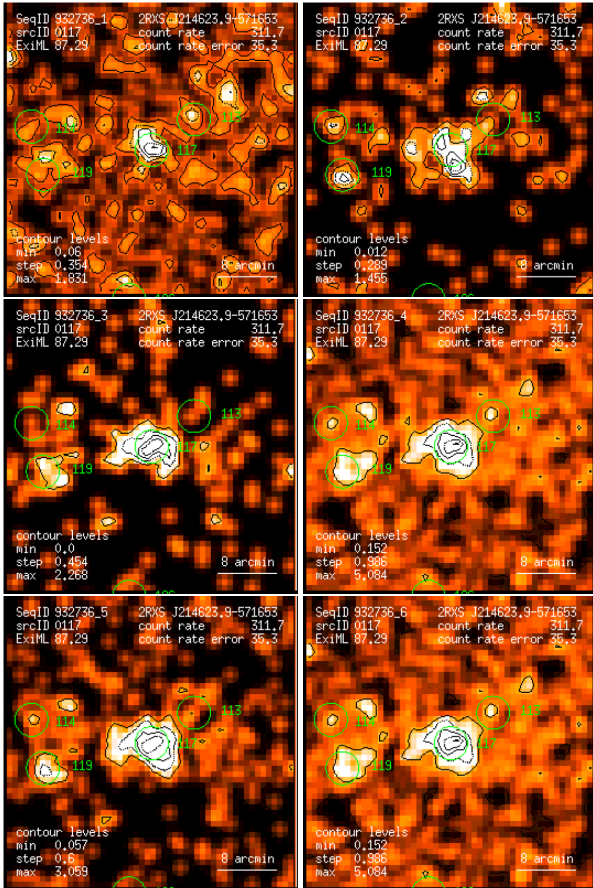
Figure 117: RASS 932736: detection 0117: band rate images, Gaussian filter: (1) PSPC channels 11 – 41, (2) 52 – 90, (3) 91 – 201, (4) 11 – 235, (5) 52 – 201, (6) 11 – 201. Broad band rates in counts/ks. Band rate contour levels in counts/ks/arcmin 2 .
