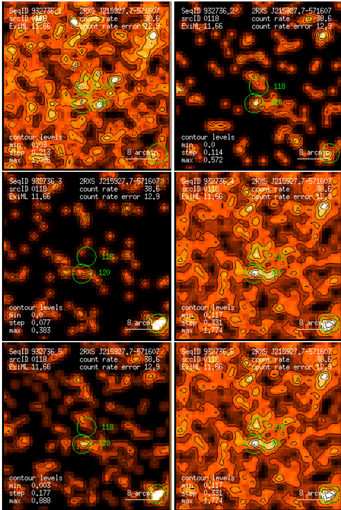
Figure 118: RASS 932736: detection 0118: band rate images, Gaussian filter: (1) PSPC channels 11 – 41, (2) 52 – 90, (3) 91 – 201, (4) 11 – 235, (5) 52 – 201, (6) 11 – 201. Broad band rates in counts/ks. Band rate contour levels in counts/ks/arcmin 2 .
