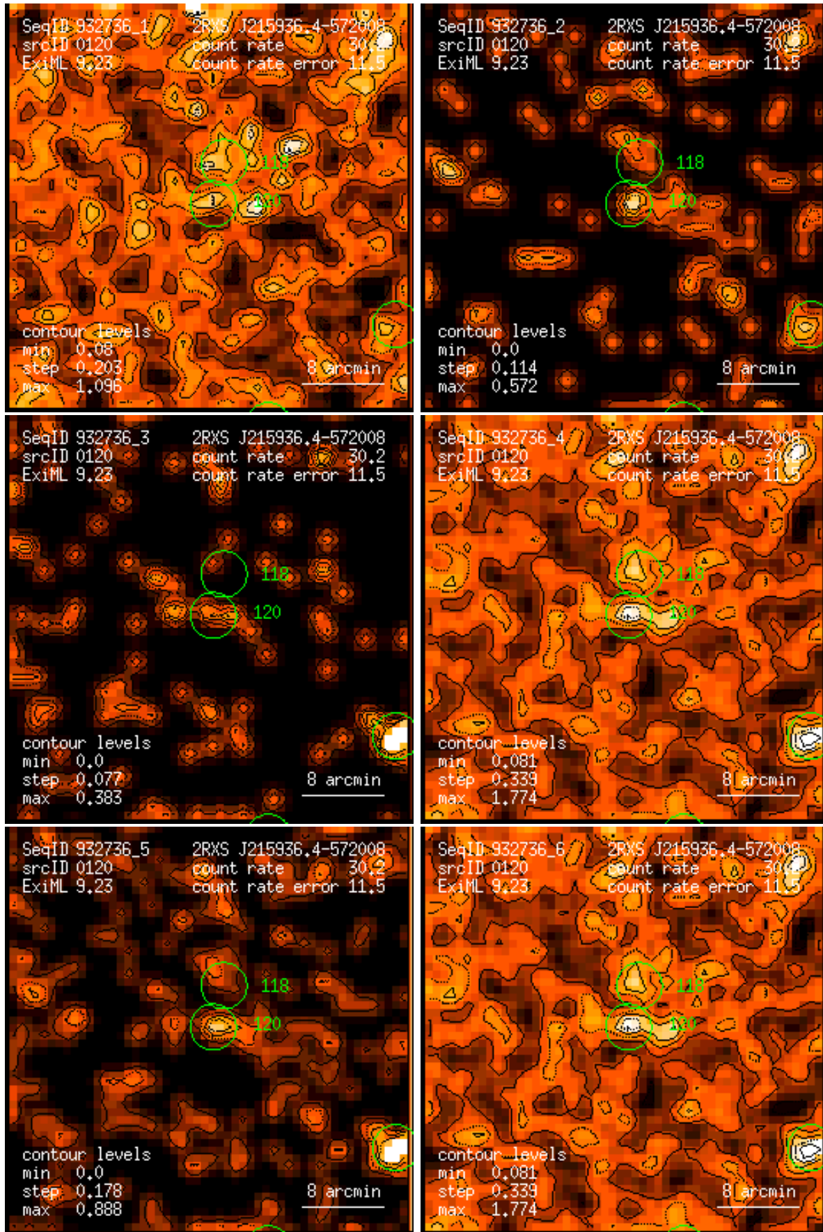
Figure 120: RASS 932736: detection 0120: band rate images, Gaussian filter: (1) PSPC channels 11 – 41, (2) 52 – 90, (3) 91 – 201, (4) 11 – 235, (5) 52 – 201, (6) 11 – 201. Broad band rates in counts/ks. Band rate contour levels in counts/ks/arcmin 2 .
