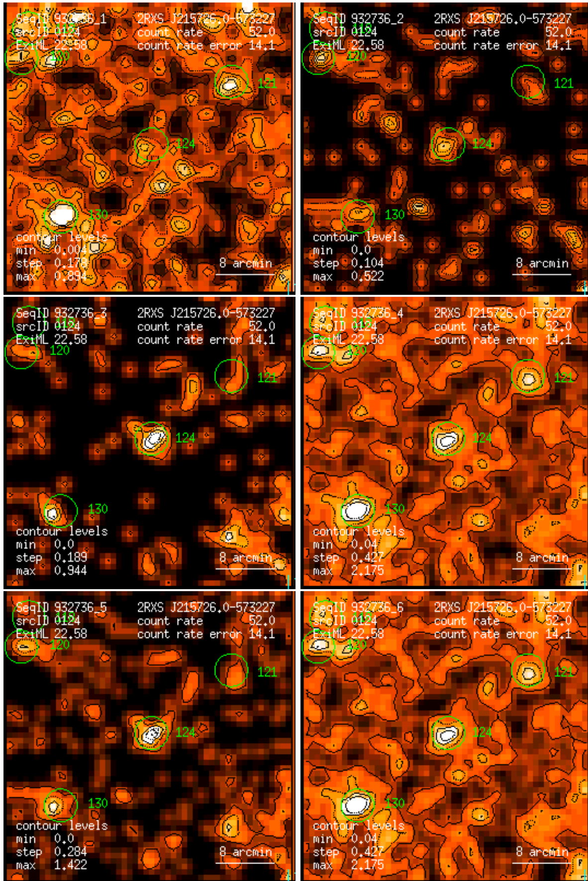
Figure 124: RASS 932736: detection 0124: band rate images, Gaussian filter: (1) PSPC channels 11 – 41, (2) 52 – 90, (3) 91 – 201, (4) 11 – 235, (5) 52 – 201, (6) 11 – 201. Broad band rates in counts/ks. Band rate contour levels in counts/ks/arcmin 2 .
