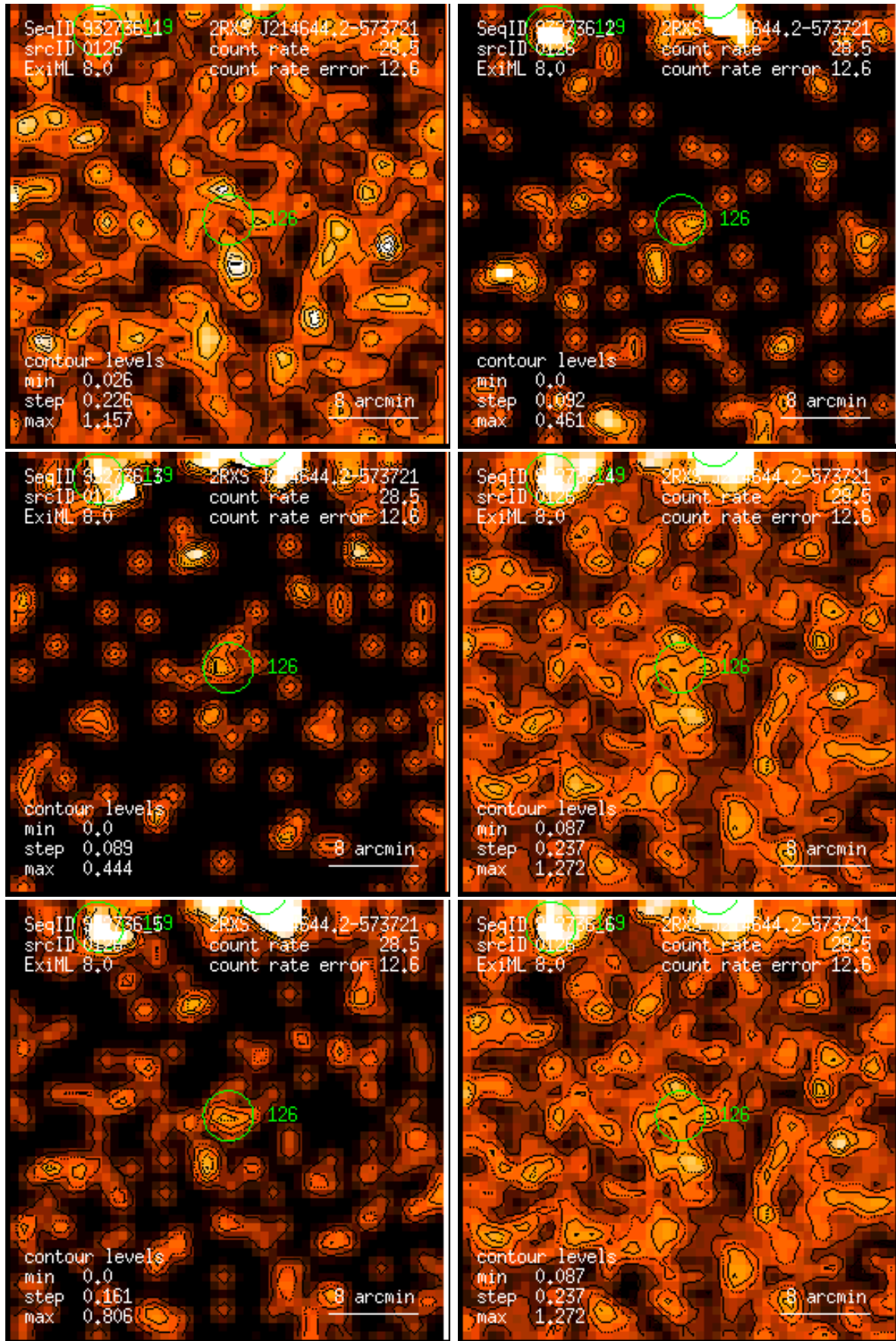
Figure 126: RASS 932736: detection 0126: band rate images, Gaussian filter: (1) PSPC channels 11 – 41, (2) 52 – 90, (3) 91 – 201, (4) 11 – 235, (5) 52 – 201, (6) 11 – 201. Broad band rates in counts/ks. Band rate contour levels in counts/ks/arcmin 2 .
