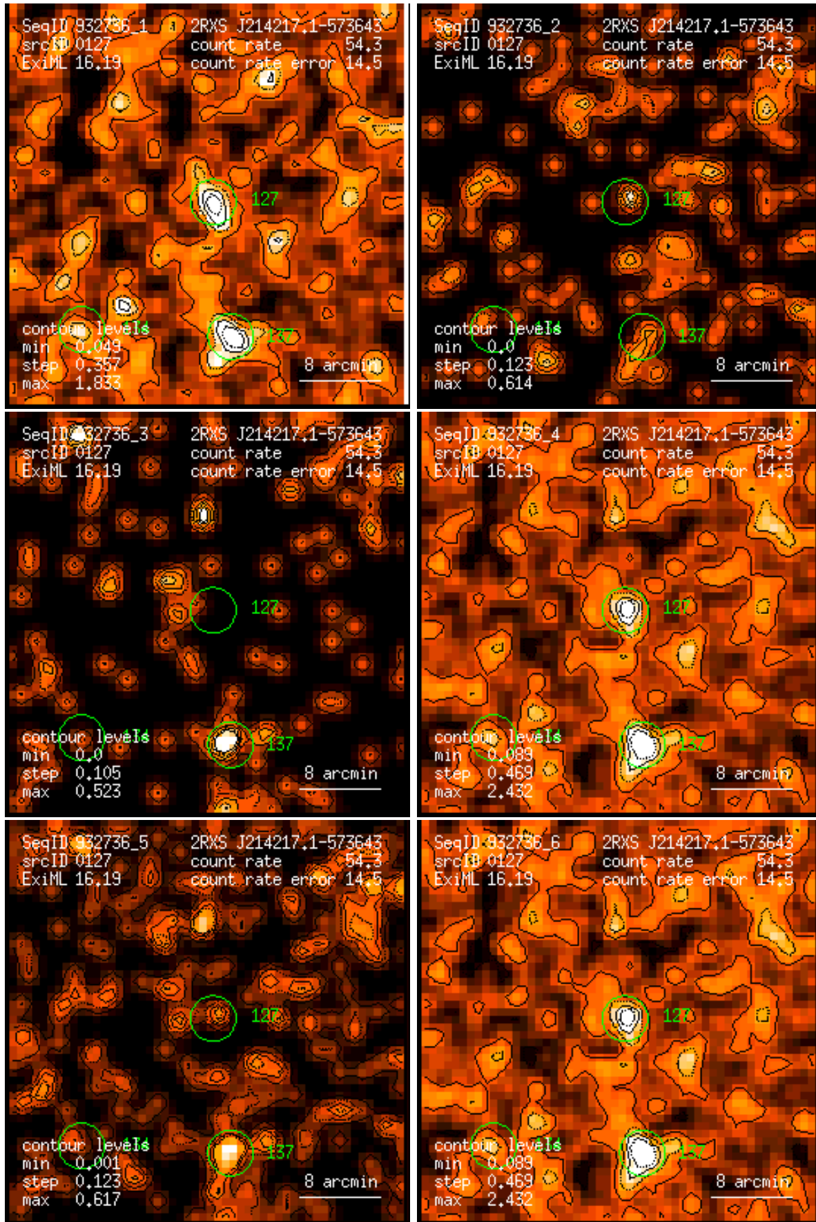
Figure 127: RASS 932736: detection 0127: band rate images, Gaussian filter: (1) PSPC channels 11 – 41, (2) 52 – 90, (3) 91 – 201, (4) 11 – 235, (5) 52 – 201, (6) 11 – 201. Broad band rates in counts/ks. Band rate contour levels in counts/ks/arcmin 2 .
