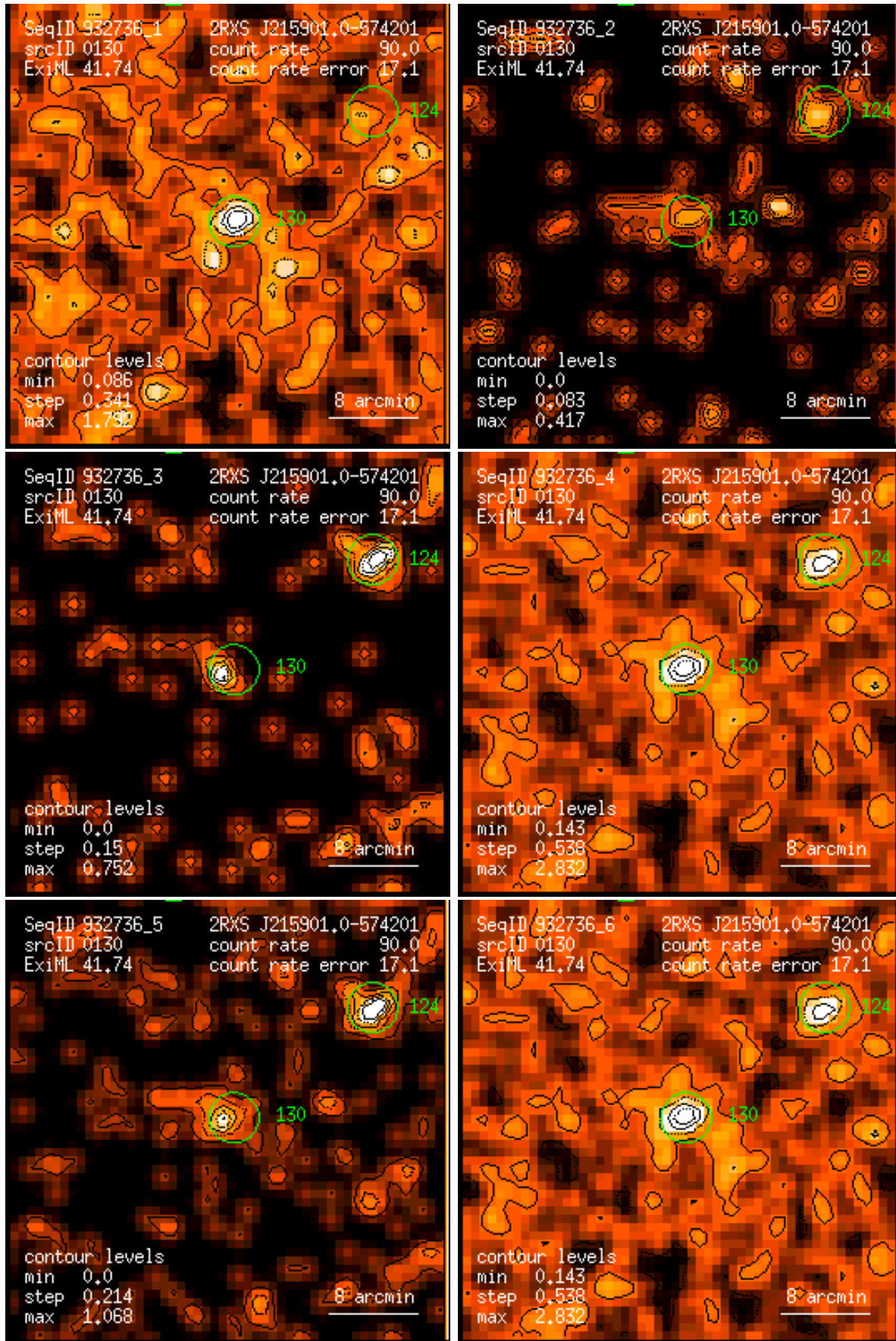
Figure 130: RASS 932736: detection 0130: band rate images, Gaussian filter: (1) PSPC channels 11 – 41, (2) 52 – 90, (3) 91 – 201, (4) 11 – 235, (5) 52 – 201, (6) 11 – 201. Broad band rates in counts/ks. Band rate contour levels in counts/ks/arcmin 2 .
