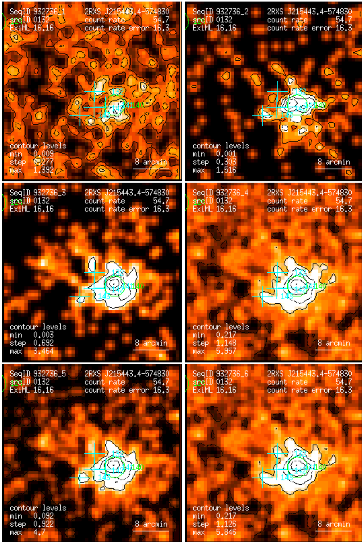
Figure 132: RASS 932736: detection 0132: band rate images, Gaussian filter: (1) PSPC channels 11 – 41, (2) 52 – 90, (3) 91 – 201, (4) 11 – 235, (5) 52 – 201, (6) 11 – 201. Broad band rates in counts/ks. Band rate contour levels in counts/ks/arcmin 2 .
