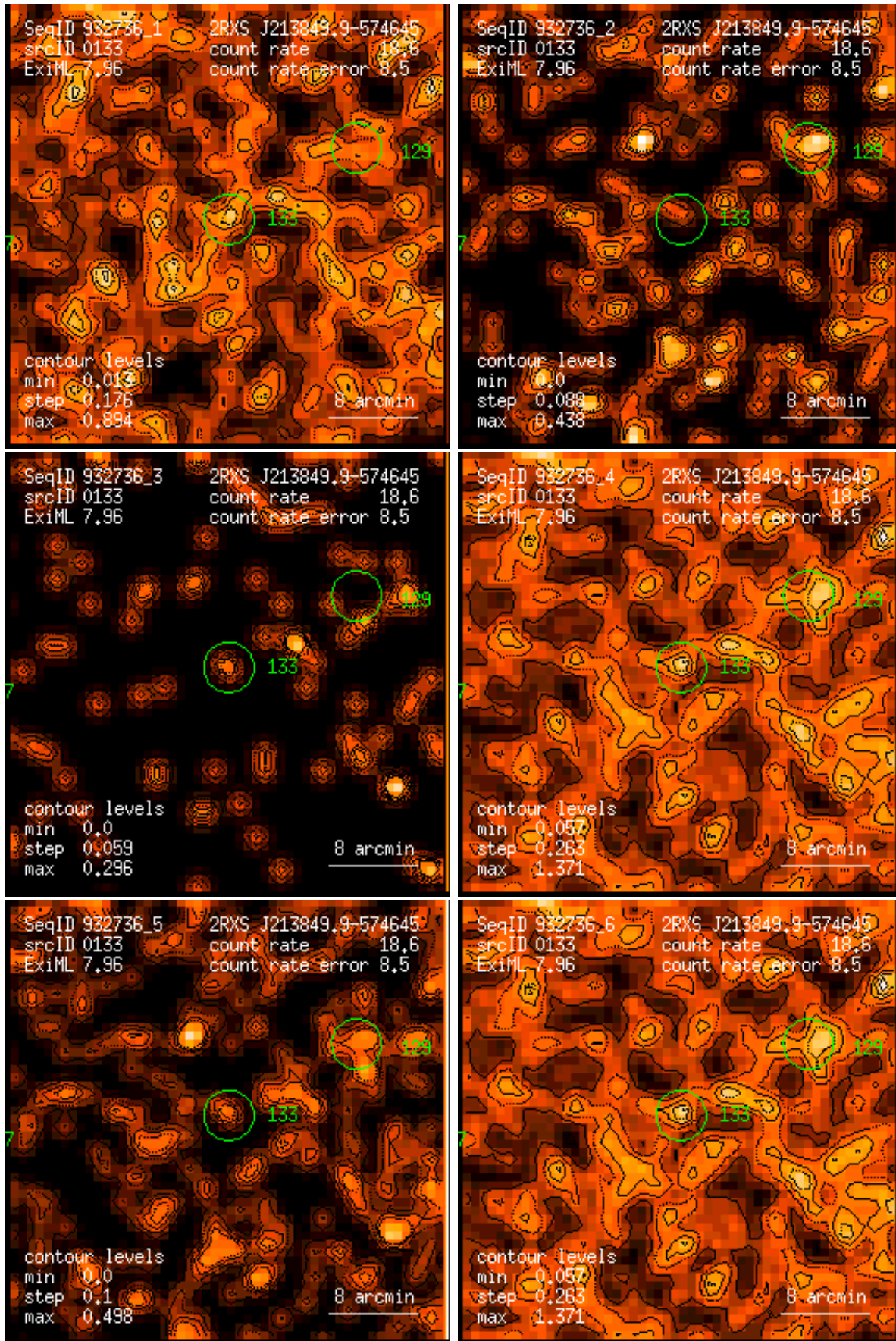
Figure 133: RASS 932736: detection 0133: band rate images, Gaussian filter: (1) PSPC channels 11 – 41, (2) 52 – 90, (3) 91 – 201, (4) 11 – 235, (5) 52 – 201, (6) 11 – 201. Broad band rates in counts/ks. Band rate contour levels in counts/ks/arcmin 2 .
