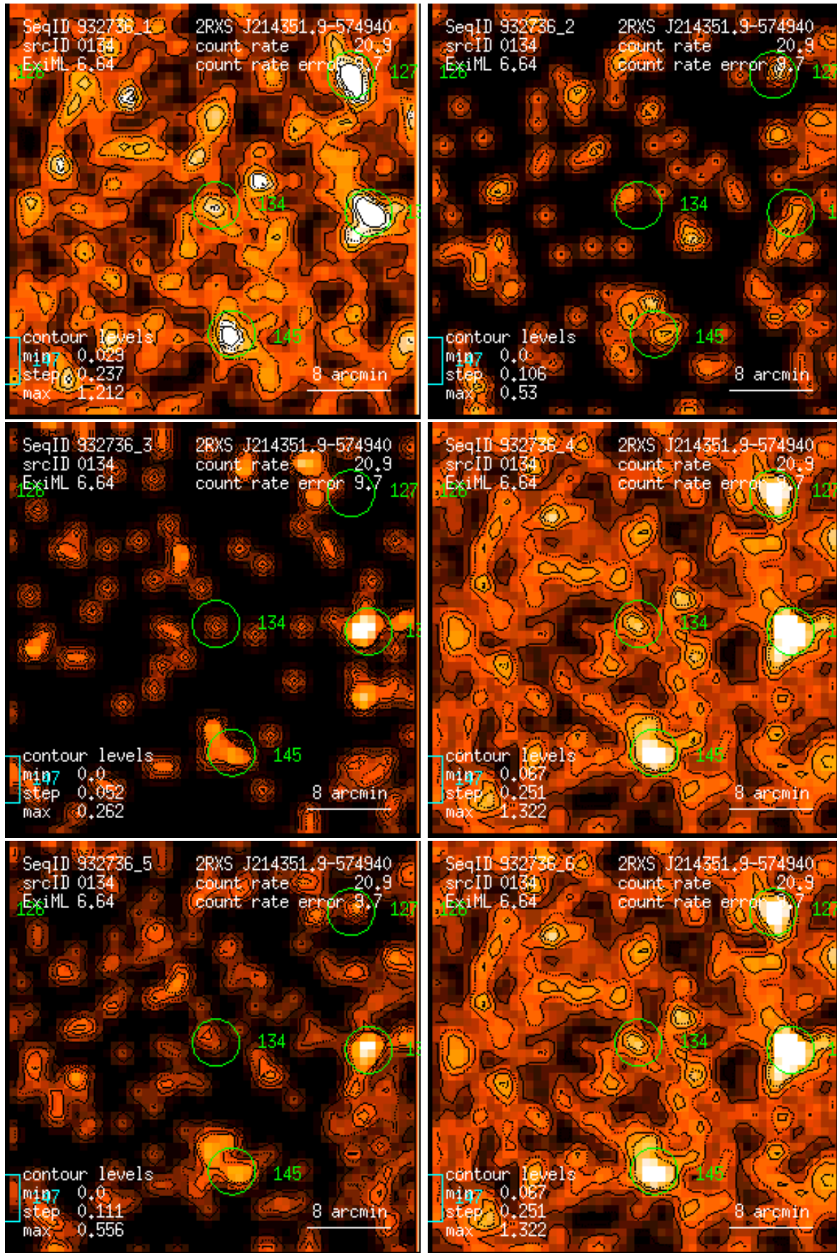
Figure 134: RASS 932736: detection 0134: band rate images, Gaussian filter: (1) PSPC channels 11 – 41, (2) 52 – 90, (3) 91 – 201, (4) 11 – 235, (5) 52 – 201, (6) 11 – 201. Broad band rates in counts/ks. Band rate contour levels in counts/ks/arcmin 2 .
