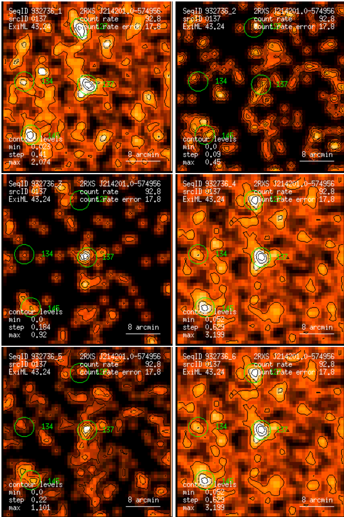
Figure 137: RASS 932736: detection 0137: band rate images, Gaussian filter: (1) PSPC channels 11 – 41, (2) 52 – 90, (3) 91 – 201, (4) 11 – 235, (5) 52 – 201, (6) 11 – 201. Broad band rates in counts/ks. Band rate contour levels in counts/ks/arcmin 2 .
