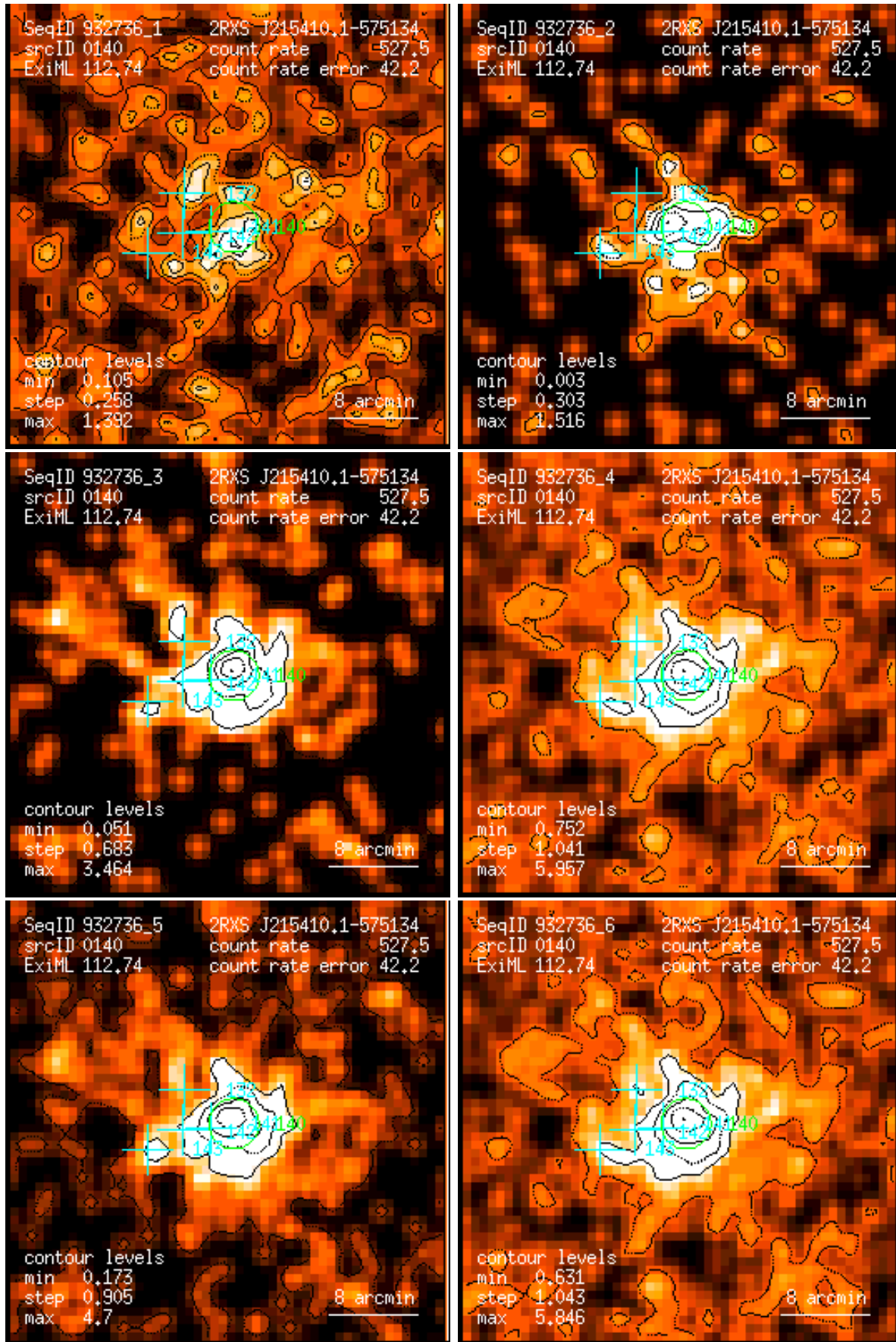
Figure 140: RASS 932736: detection 0140: band rate images, Gaussian filter: (1) PSPC channels 11 – 41, (2) 52 – 90, (3) 91 – 201, (4) 11 – 235, (5) 52 – 201, (6) 11 – 201. Broad band rates in counts/ks. Band rate contour levels in counts/ks/arcmin 2 .
