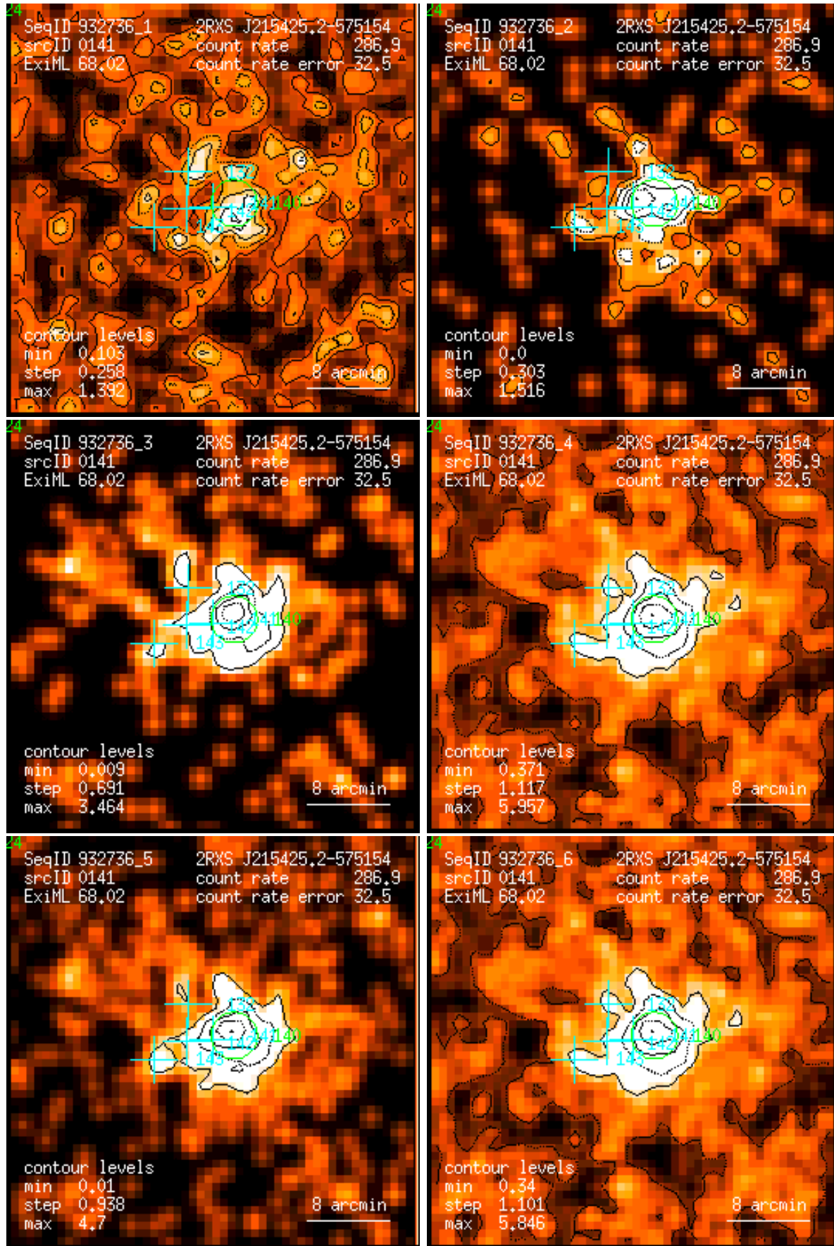
Figure 141: RASS 932736: detection 0141: band rate images, Gaussian filter: (1) PSPC channels 11 – 41, (2) 52 – 90, (3) 91 – 201, (4) 11 – 235, (5) 52 – 201, (6) 11 – 201. Broad band rates in counts/ks. Band rate contour levels in counts/ks/arcmin 2 .
