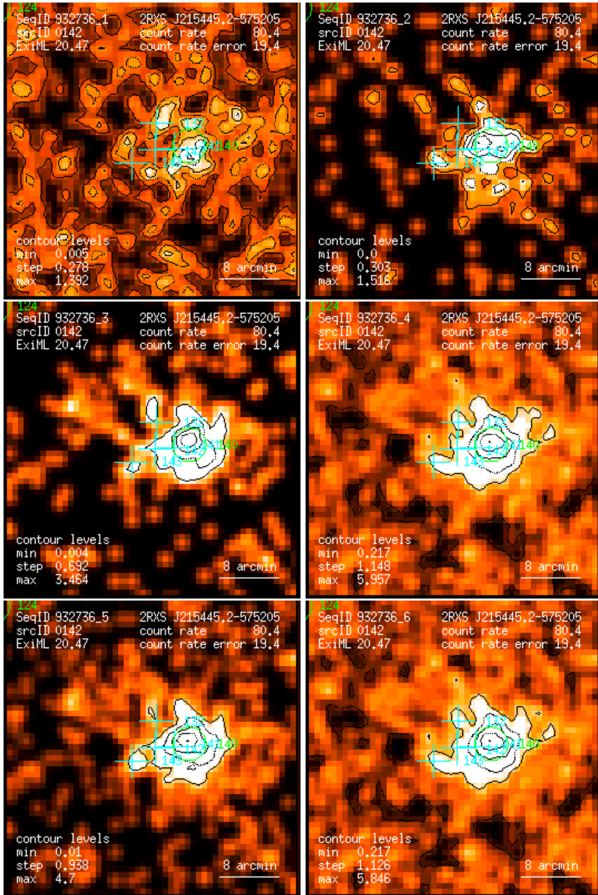
Figure 142: RASS 932736: detection 0142: band rate images, Gaussian filter: (1) PSPC channels 11 – 41, (2) 52 – 90, (3) 91 – 201, (4) 11 – 235, (5) 52 – 201, (6) 11 – 201. Broad band rates in counts/ks. Band rate contour levels in counts/ks/arcmin 2 .
