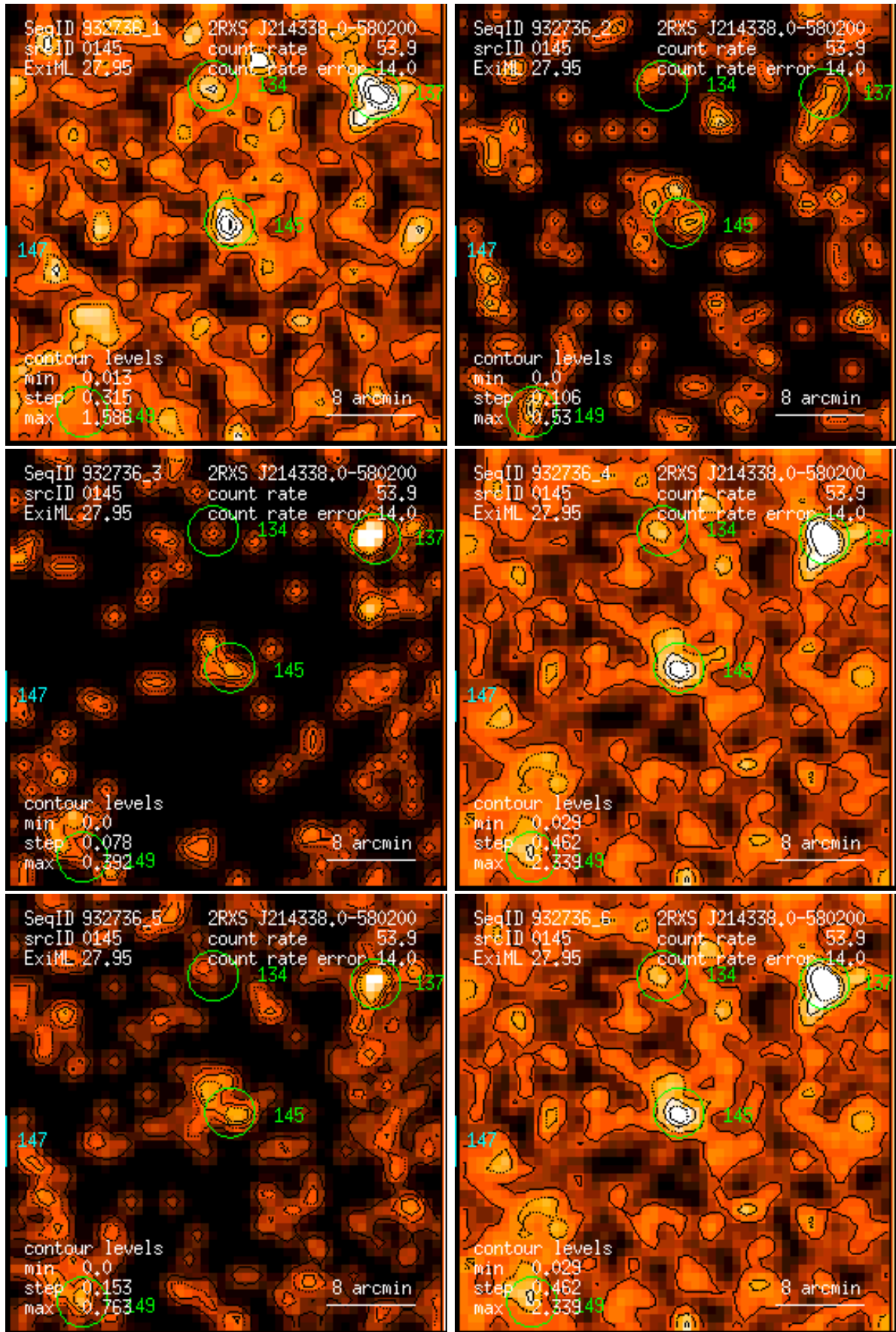
Figure 145: RASS 932736: detection 0145: band rate images, Gaussian filter: (1) PSPC channels 11 – 41, (2) 52 – 90, (3) 91 – 201, (4) 11 – 235, (5) 52 – 201, (6) 11 – 201. Broad band rates in counts/ks. Band rate contour levels in counts/ks/arcmin 2 .
