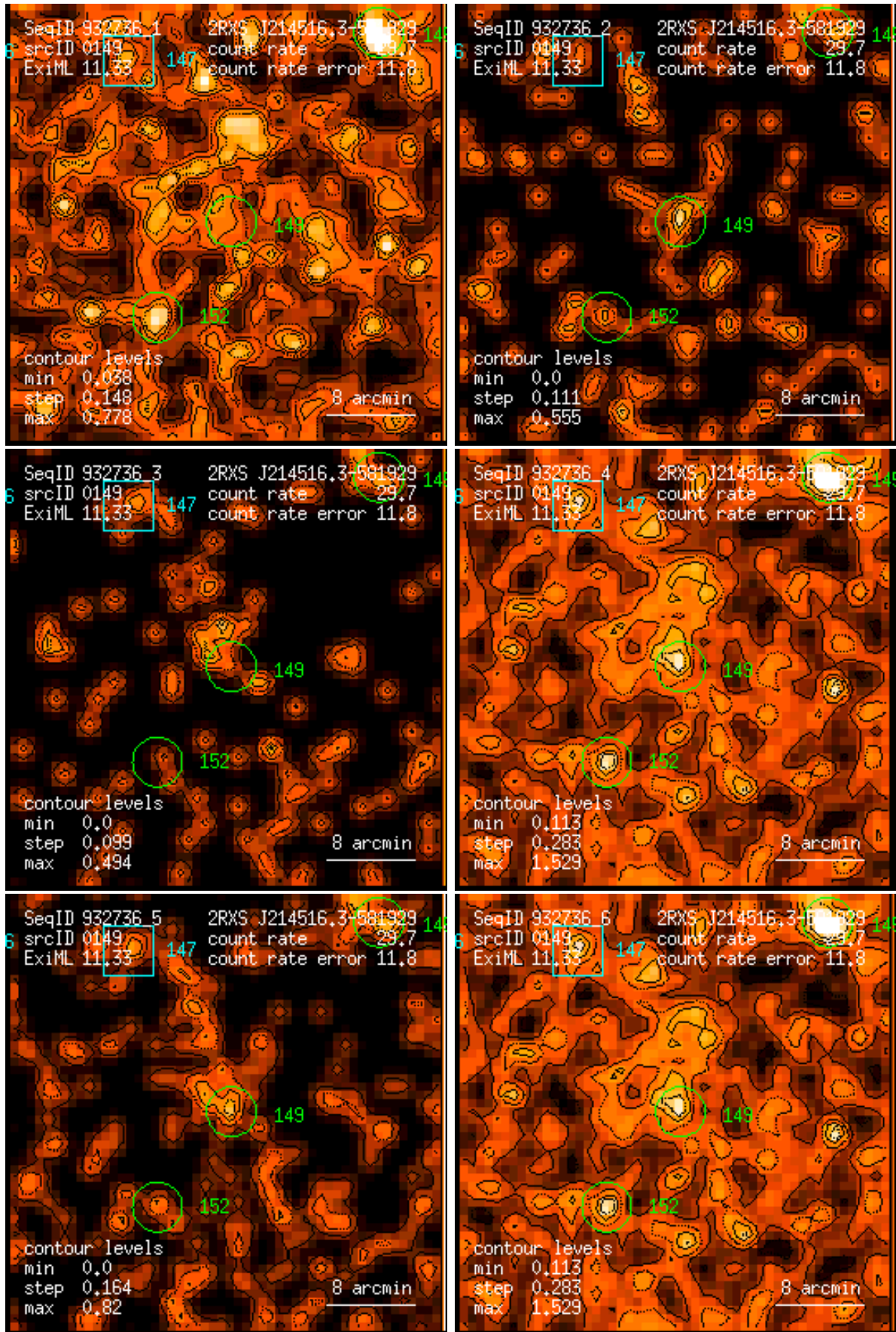
Figure 149: RASS 932736: detection 0149: band rate images, Gaussian filter: (1) PSPC channels 11 – 41, (2) 52 – 90, (3) 91 – 201, (4) 11 – 235, (5) 52 – 201, (6) 11 – 201. Broad band rates in counts/ks. Band rate contour levels in counts/ks/arcmin 2 .
