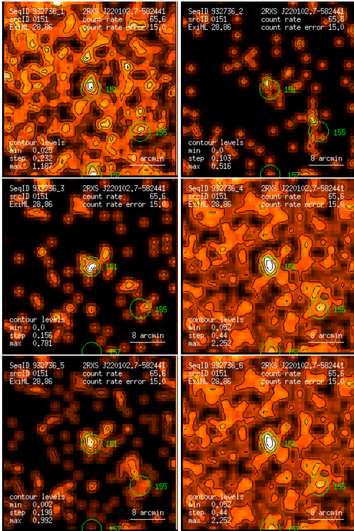
Figure 151: RASS 932736: detection 0151: band rate images, Gaussian filter: (1) PSPC channels 11 – 41, (2) 52 – 90, (3) 91 – 201, (4) 11 – 235, (5) 52 – 201, (6) 11 – 201. Broad band rates in counts/ks. Band rate contour levels in counts/ks/arcmin 2 .
