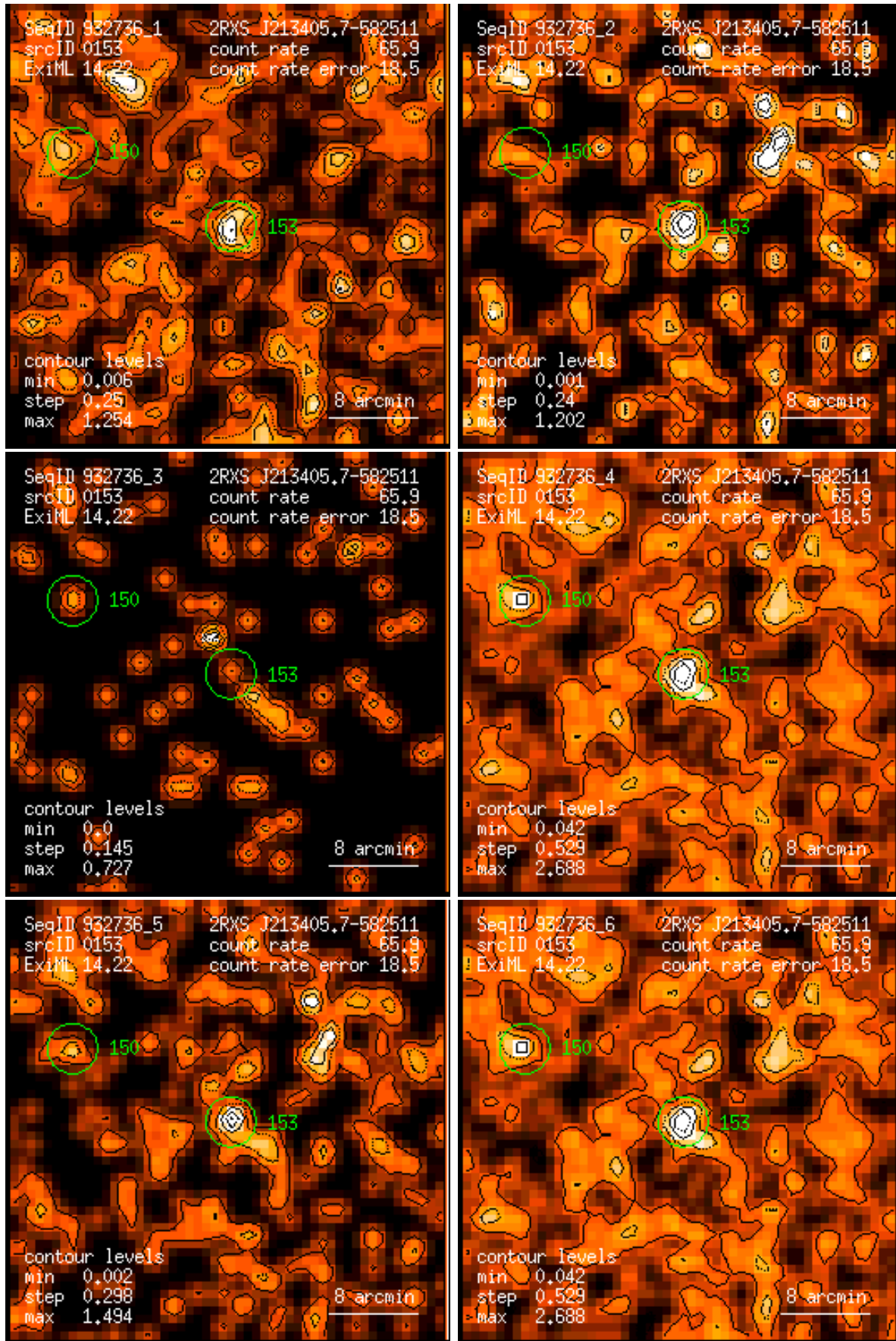
Figure 153: RASS 932736: detection 0153: band rate images, Gaussian filter: (1) PSPC channels 11 – 41, (2) 52 – 90, (3) 91 – 201, (4) 11 – 235, (5) 52 – 201, (6) 11 – 201. Broad band rates in counts/ks. Band rate contour levels in counts/ks/arcmin 2 .
