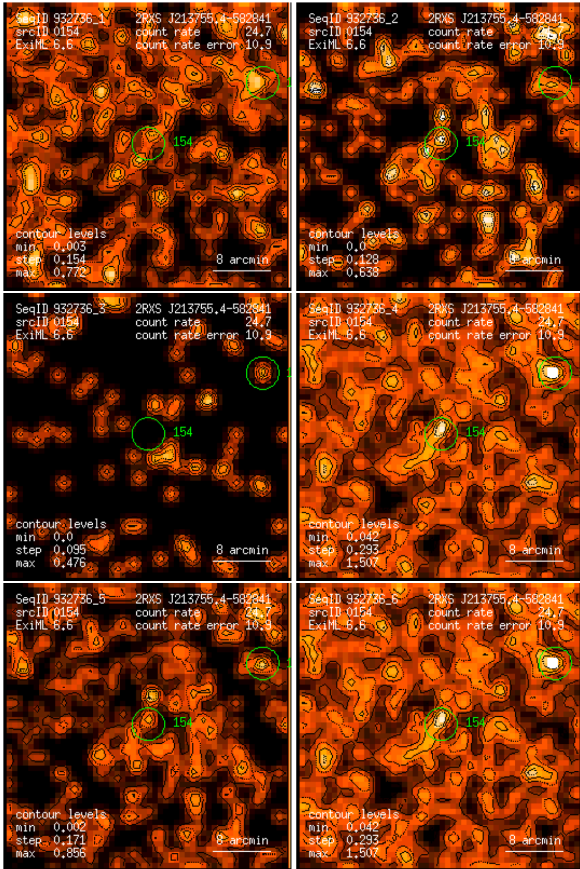
Figure 154: RASS 932736: detection 0154: band rate images, Gaussian filter: (1) PSPC channels 11 – 41, (2) 52 – 90, (3) 91 – 201, (4) 11 – 235, (5) 52 – 201, (6) 11 – 201. Broad band rates in counts/ks. Band rate contour levels in counts/ks/arcmin 2 .
