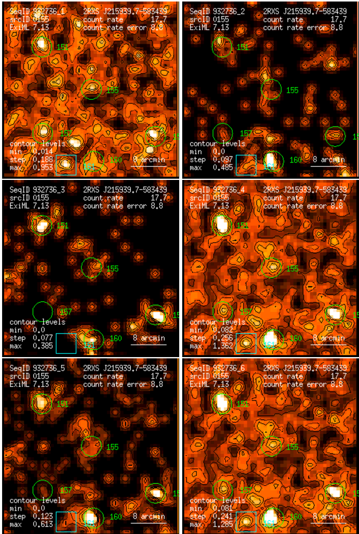
Figure 155: RASS 932736: detection 0155: band rate images, Gaussian filter: (1) PSPC channels 11 – 41, (2) 52 – 90, (3) 91 – 201, (4) 11 – 235, (5) 52 – 201, (6) 11 – 201. Broad band rates in counts/ks. Band rate contour levels in counts/ks/arcmin 2 .
