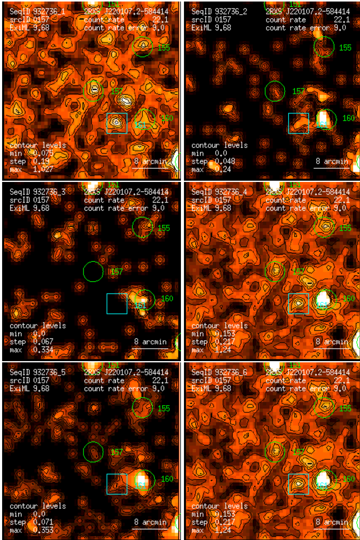
Figure 157: RASS 932736: detection 0157: band rate images, Gaussian filter: (1) PSPC channels 11 – 41, (2) 52 – 90, (3) 91 – 201, (4) 11 – 235, (5) 52 – 201, (6) 11 – 201. Broad band rates in counts/ks. Band rate contour levels in counts/ks/arcmin 2 .
