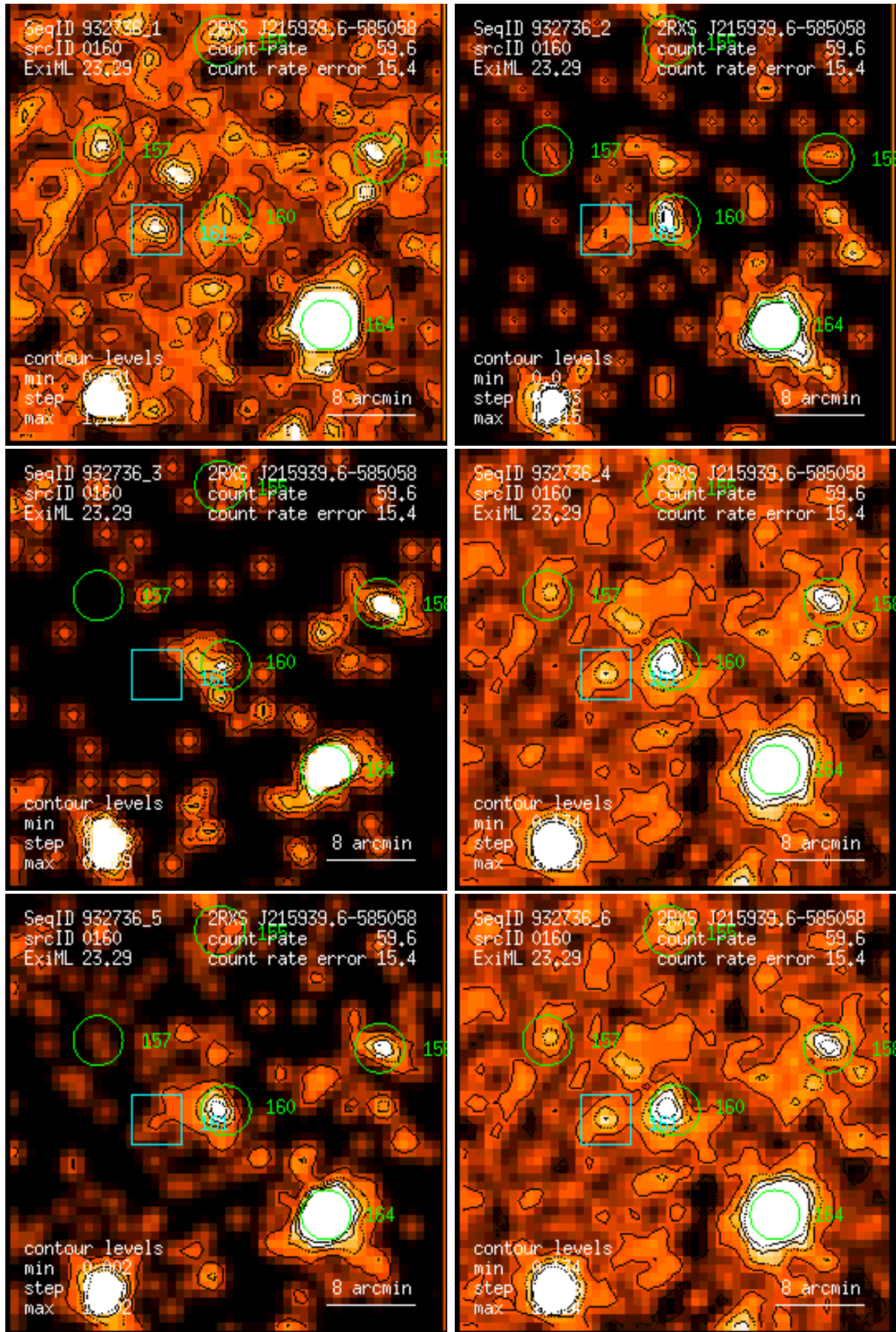
Figure 160: RASS 932736: detection 0160: band rate images, Gaussian filter: (1) PSPC channels 11 – 41, (2) 52 – 90, (3) 91 – 201, (4) 11 – 235, (5) 52 – 201, (6) 11 – 201. Broad band rates in counts/ks. Band rate contour levels in counts/ks/arcmin 2 .
