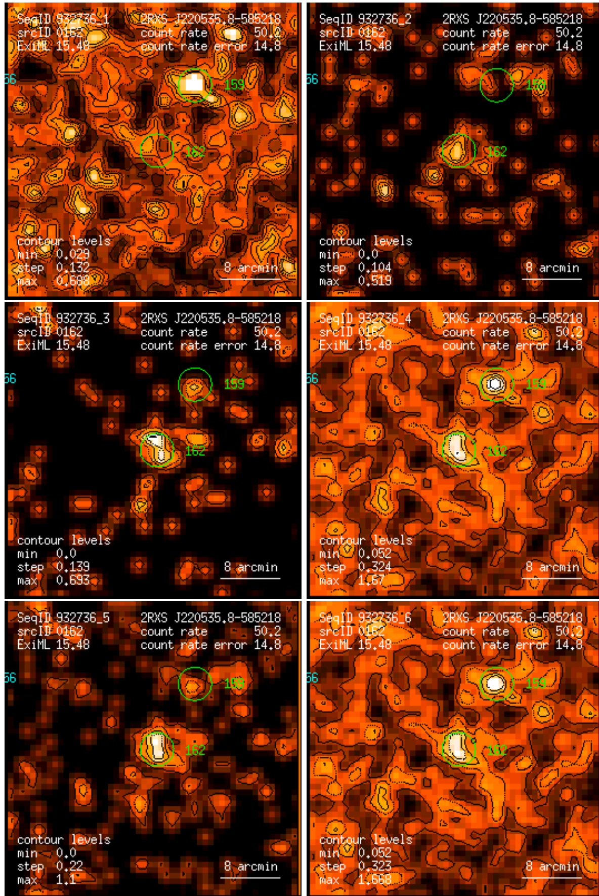
Figure 162: RASS 932736: detection 0162: band rate images, Gaussian filter: (1) PSPC channels 11 – 41, (2) 52 – 90, (3) 91 – 201, (4) 11 – 235, (5) 52 – 201, (6) 11 – 201. Broad band rates in counts/ks. Band rate contour levels in counts/ks/arcmin 2 .
