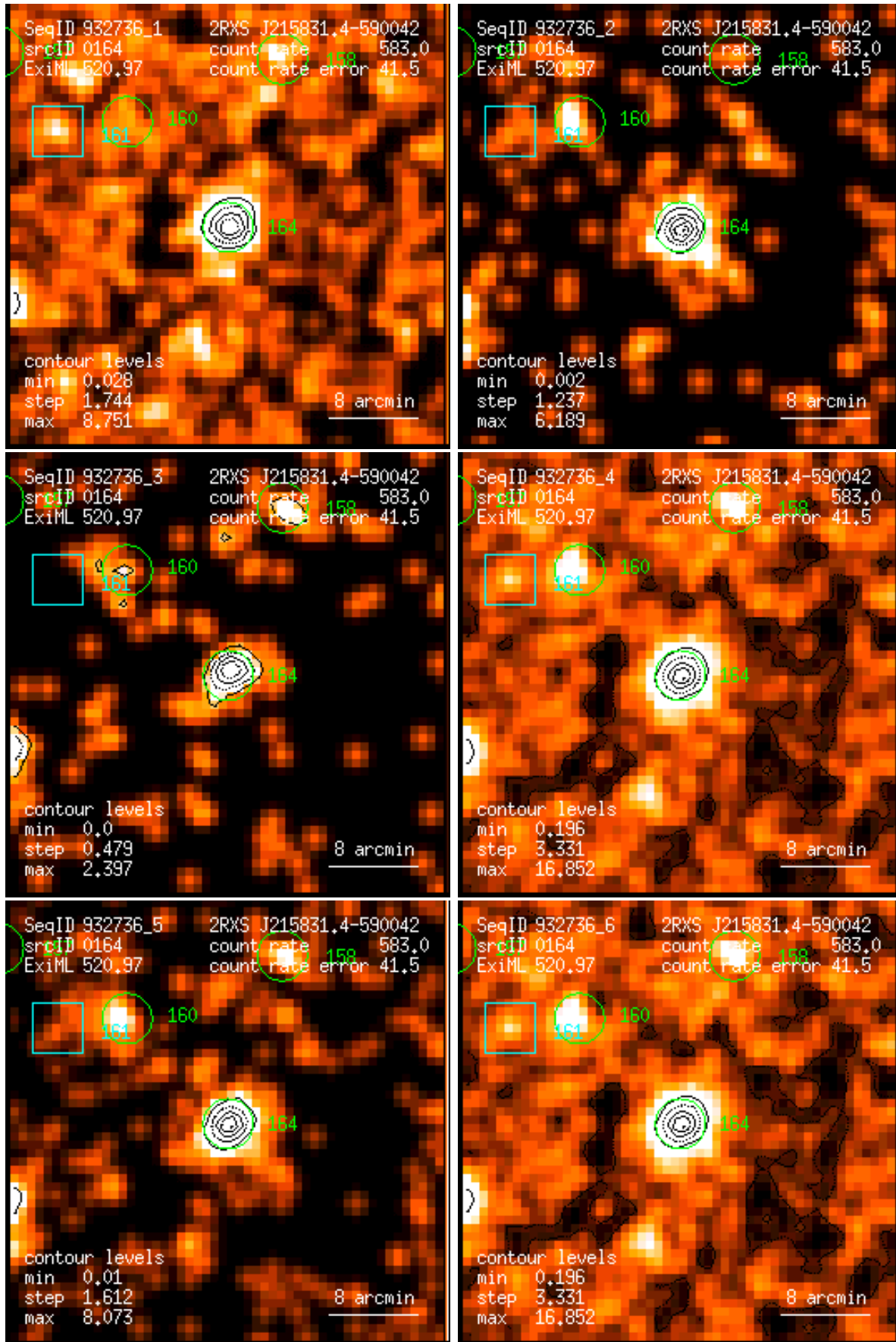
Figure 164: RASS 932736: detection 0164: band rate images, Gaussian filter: (1) PSPC channels 11 – 41, (2) 52 – 90, (3) 91 – 201, (4) 11 – 235, (5) 52 – 201, (6) 11 – 201. Broad band rates in counts/ks. Band rate contour levels in counts/ks/arcmin 2 .
