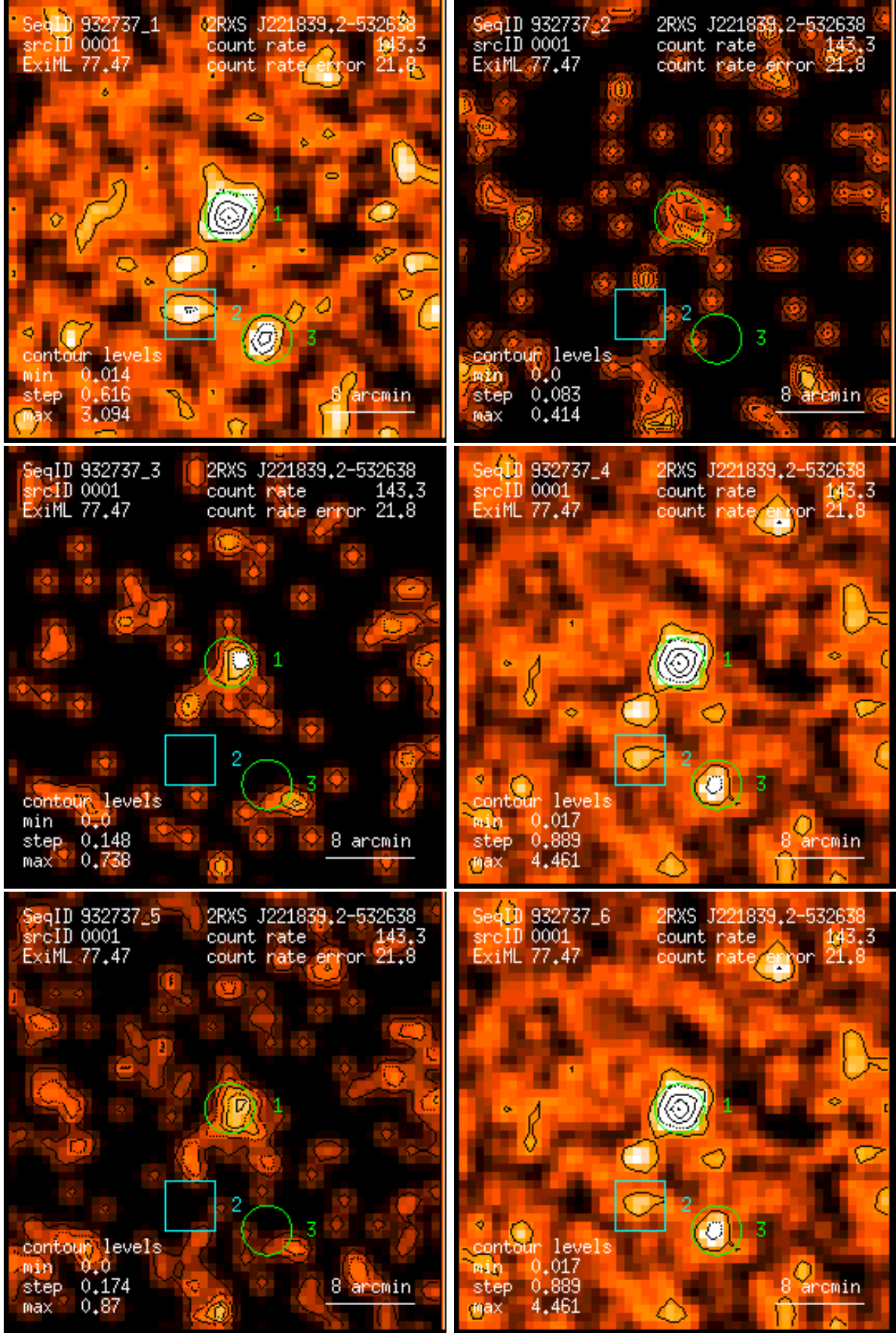
Figure 1: RASS 932737: detection 0001: band rate images, Gaussian filter: (1) PSPC channels 11 – 41, (2) 52 – 90, (3) 91 – 201, (4) 11 – 235, (5) 52 – 201, (6) 11 – 201. Broad band rates in counts/ks. Band rate contour levels in counts/ks/arcmin 2 .
