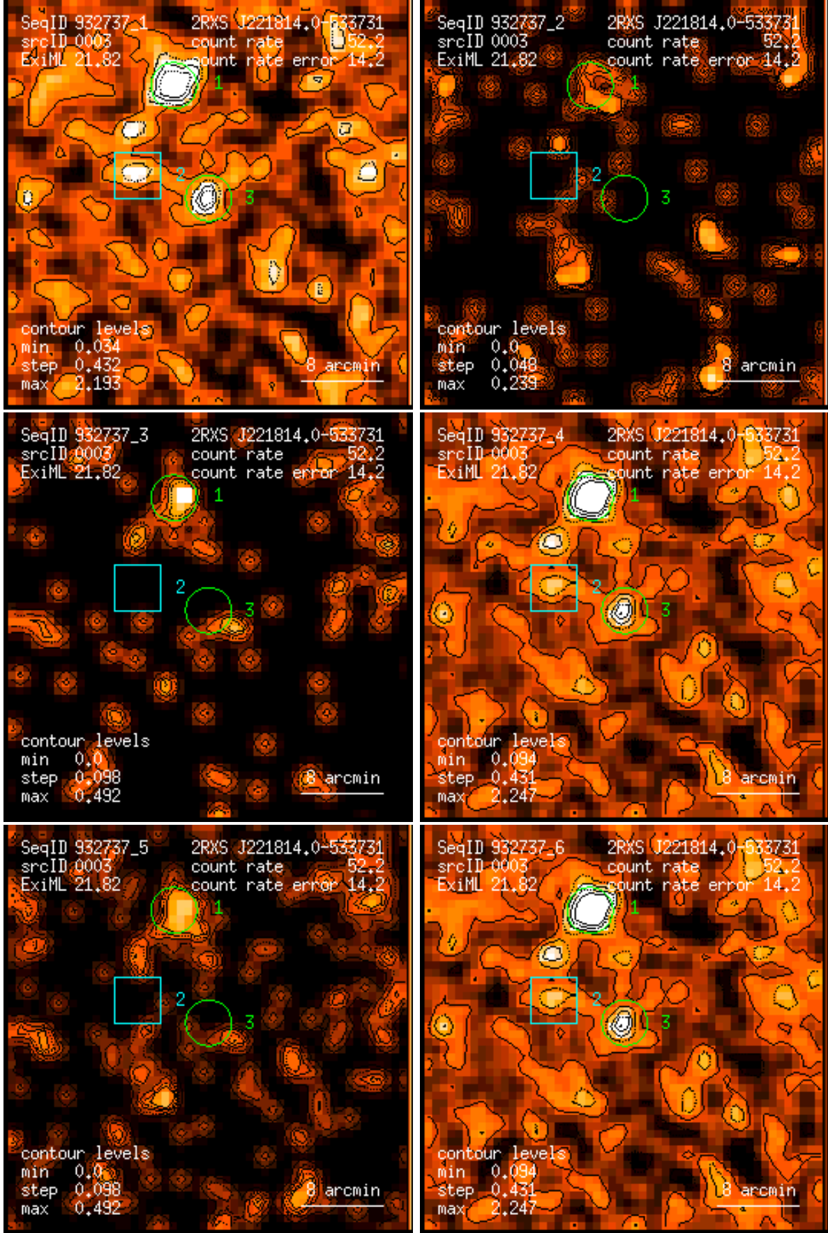
Figure 3: RASS 932737: detection 0003: band rate images, Gaussian filter: (1) PSPC channels 11 – 41, (2) 52 – 90, (3) 91 – 201, (4) 11 – 235, (5) 52 – 201, (6) 11 – 201. Broad band rates in counts/ks. Band rate contour levels in counts/ks/arcmin 2 .
