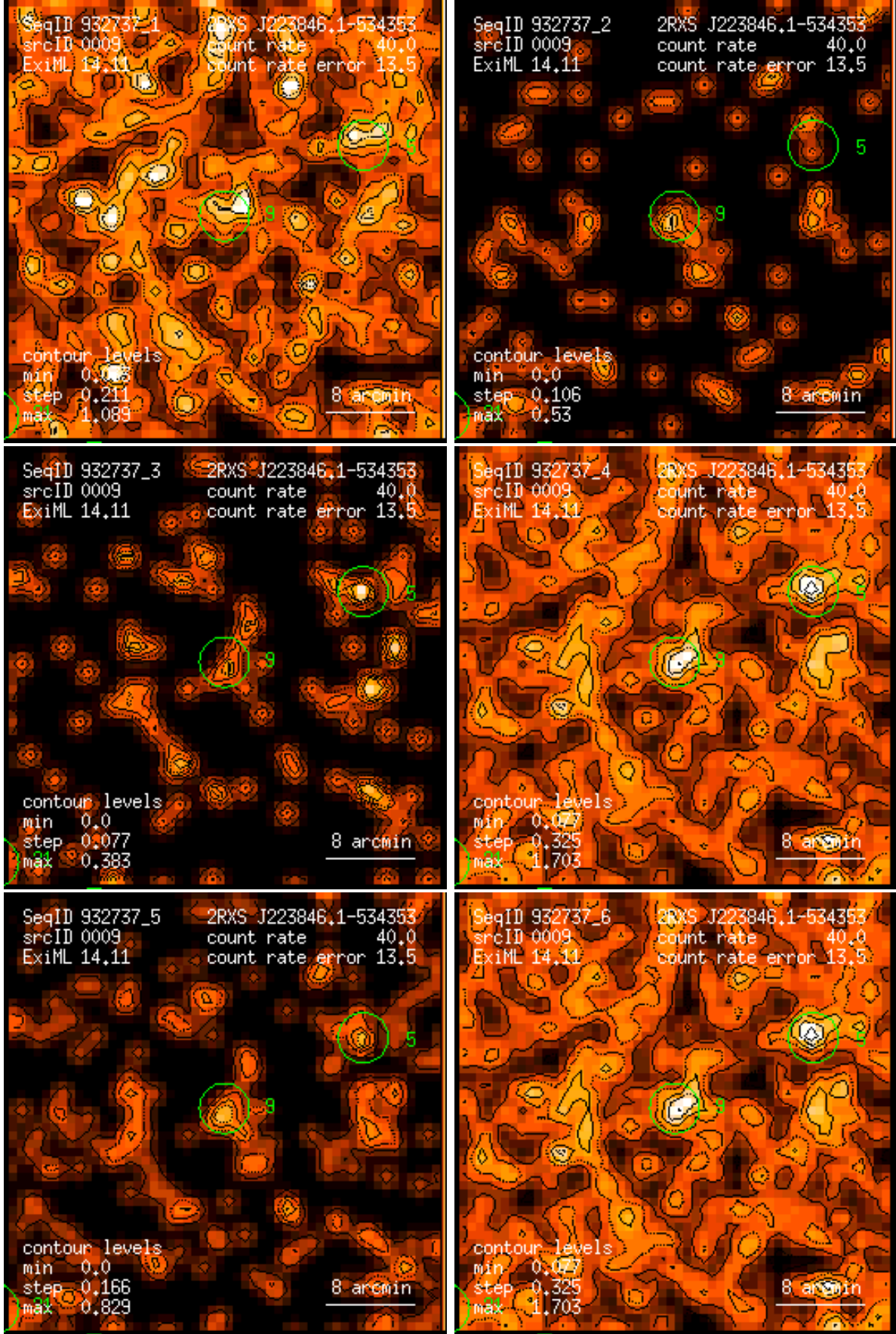
Figure 9: RASS 932737: detection 0009: band rate images, Gaussian filter: (1) PSPC channels 11 – 41, (2) 52 – 90, (3) 91 – 201, (4) 11 – 235, (5) 52 – 201, (6) 11 – 201. Broad band rates in counts/ks. Band rate contour levels in counts/ks/arcmin 2 .
