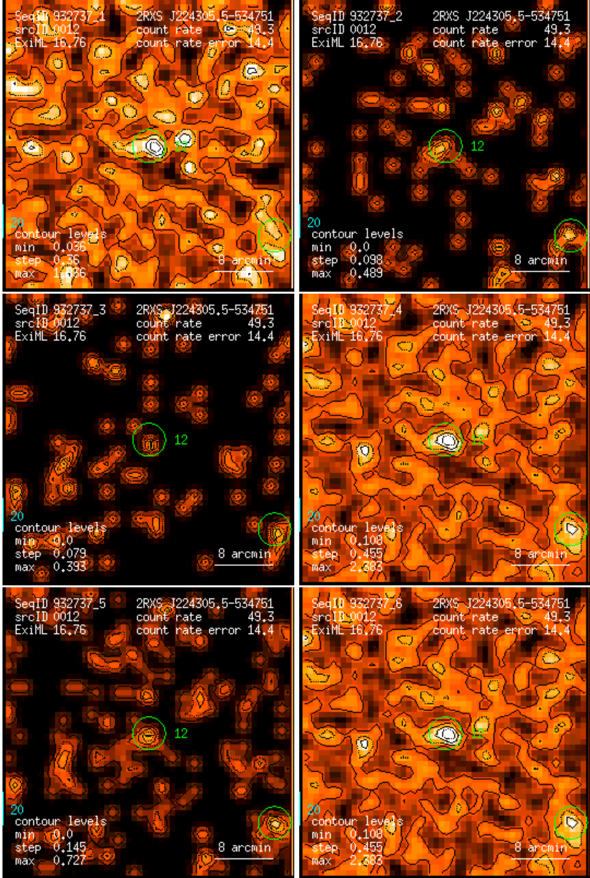
Figure 12: RASS 932737: detection 0012: band rate images, Gaussian filter: (1) PSPC channels 11 – 41, (2) 52 – 90, (3) 91 – 201, (4) 11 – 235, (5) 52 – 201, (6) 11 – 201. Broad band rates in counts/ks. Band rate contour levels in counts/ks/arcmin 2 .
