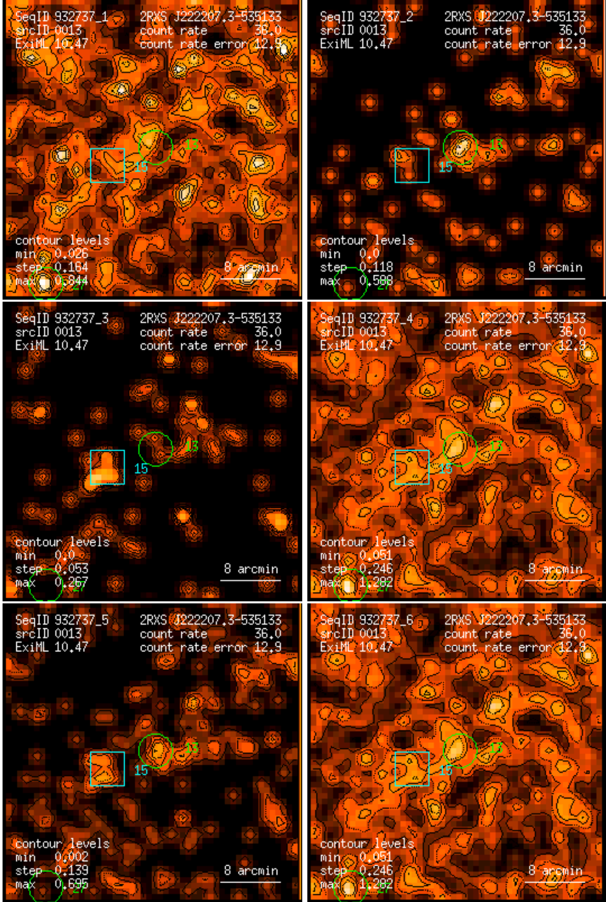
Figure 13: RASS 932737: detection 0013: band rate images, Gaussian filter: (1) PSPC channels 11 – 41, (2) 52 – 90, (3) 91 – 201, (4) 11 – 235, (5) 52 – 201, (6) 11 – 201. Broad band rates in counts/ks. Band rate contour levels in counts/ks/arcmin 2 .
