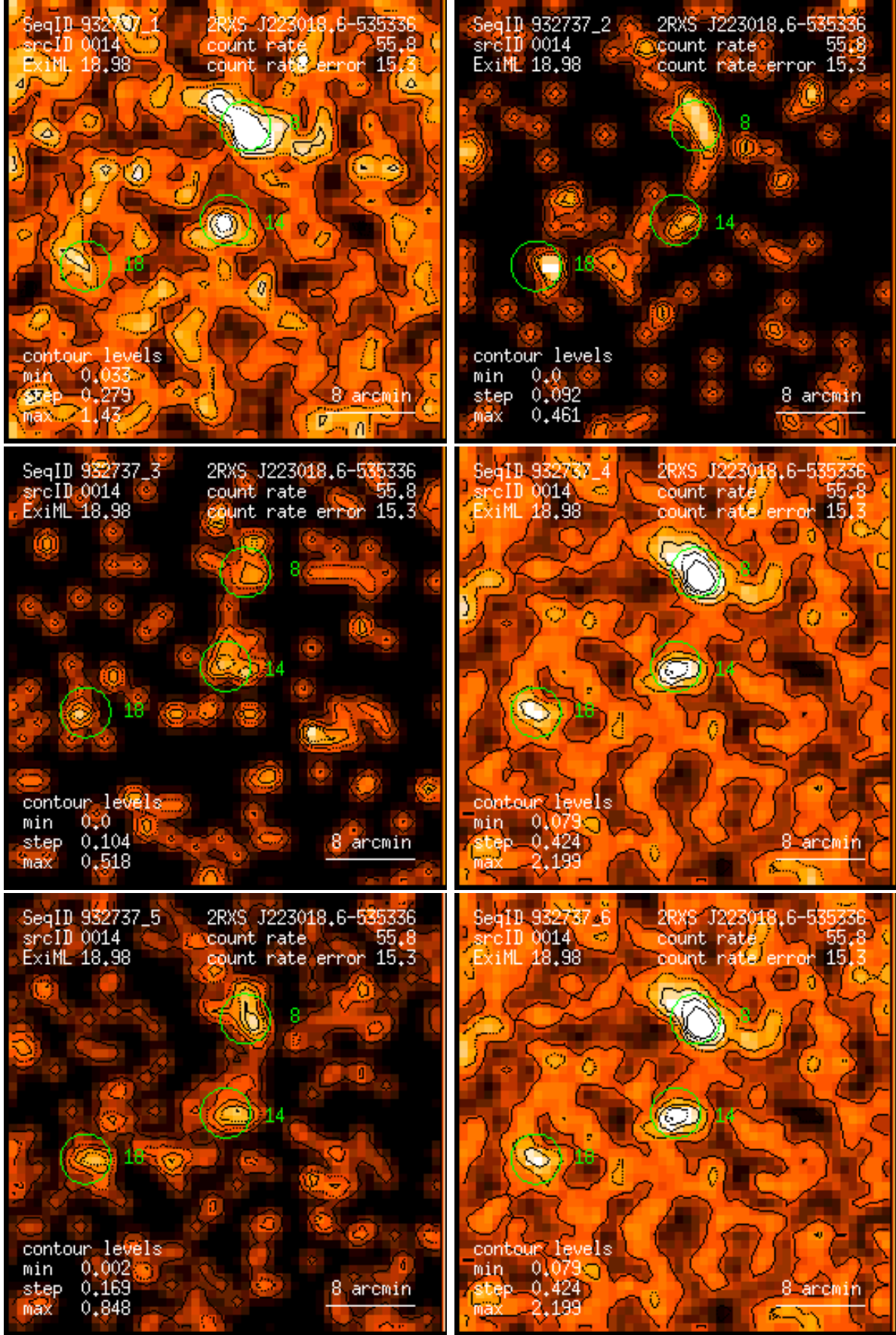
Figure 14: RASS 932737: detection 0014: band rate images, Gaussian filter: (1) PSPC channels 11 – 41, (2) 52 – 90, (3) 91 – 201, (4) 11 – 235, (5) 52 – 201, (6) 11 – 201. Broad band rates in counts/ks. Band rate contour levels in counts/ks/arcmin 2 .
