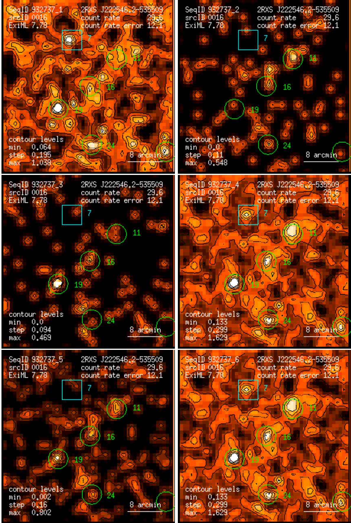
Figure 16: RASS 932737: detection 0016: band rate images, Gaussian filter: (1) PSPC channels 11 – 41, (2) 52 – 90, (3) 91 – 201, (4) 11 – 235, (5) 52 – 201, (6) 11 – 201. Broad band rates in counts/ks. Band rate contour levels in counts/ks/arcmin 2 .
