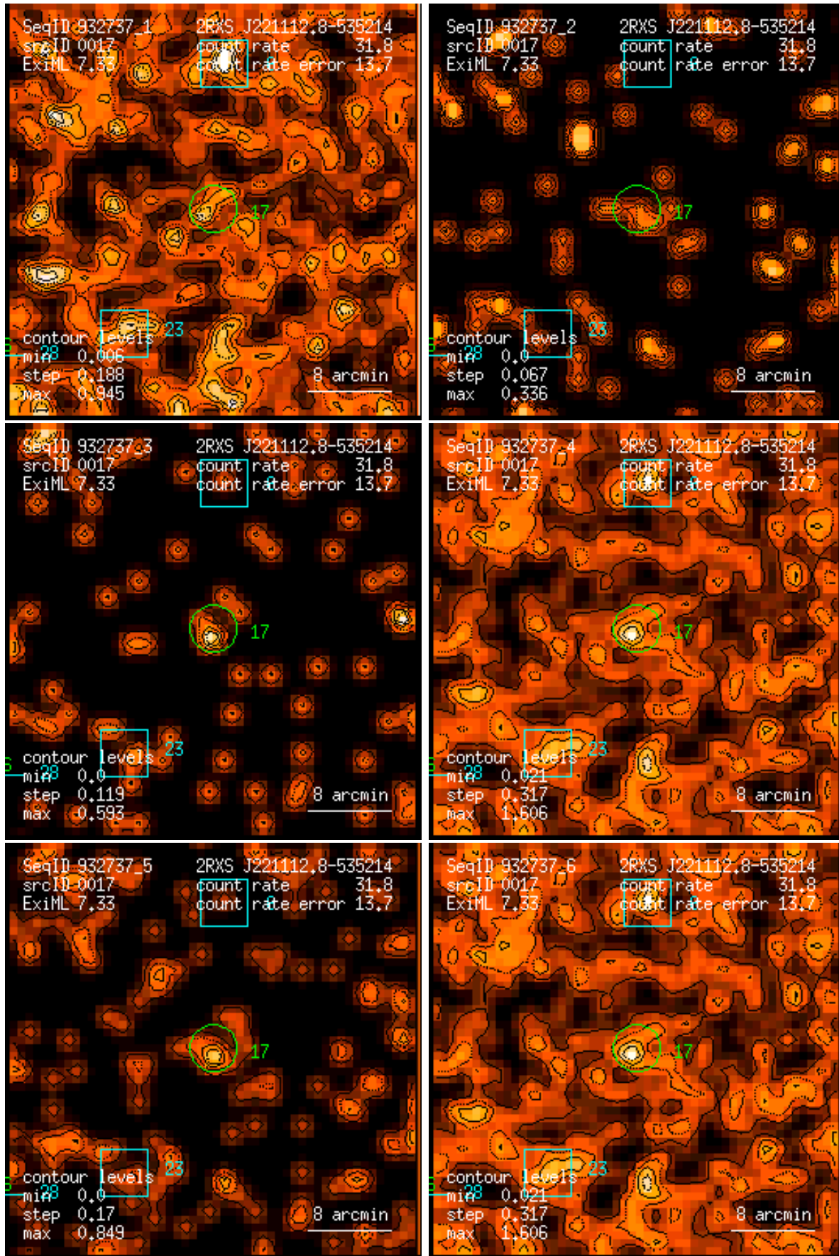
Figure 17: RASS 932737: detection 0017: band rate images, Gaussian filter: (1) PSPC channels 11 – 41, (2) 52 – 90, (3) 91 – 201, (4) 11 – 235, (5) 52 – 201, (6) 11 – 201. Broad band rates in counts/ks. Band rate contour levels in counts/ks/arcmin 2 .
