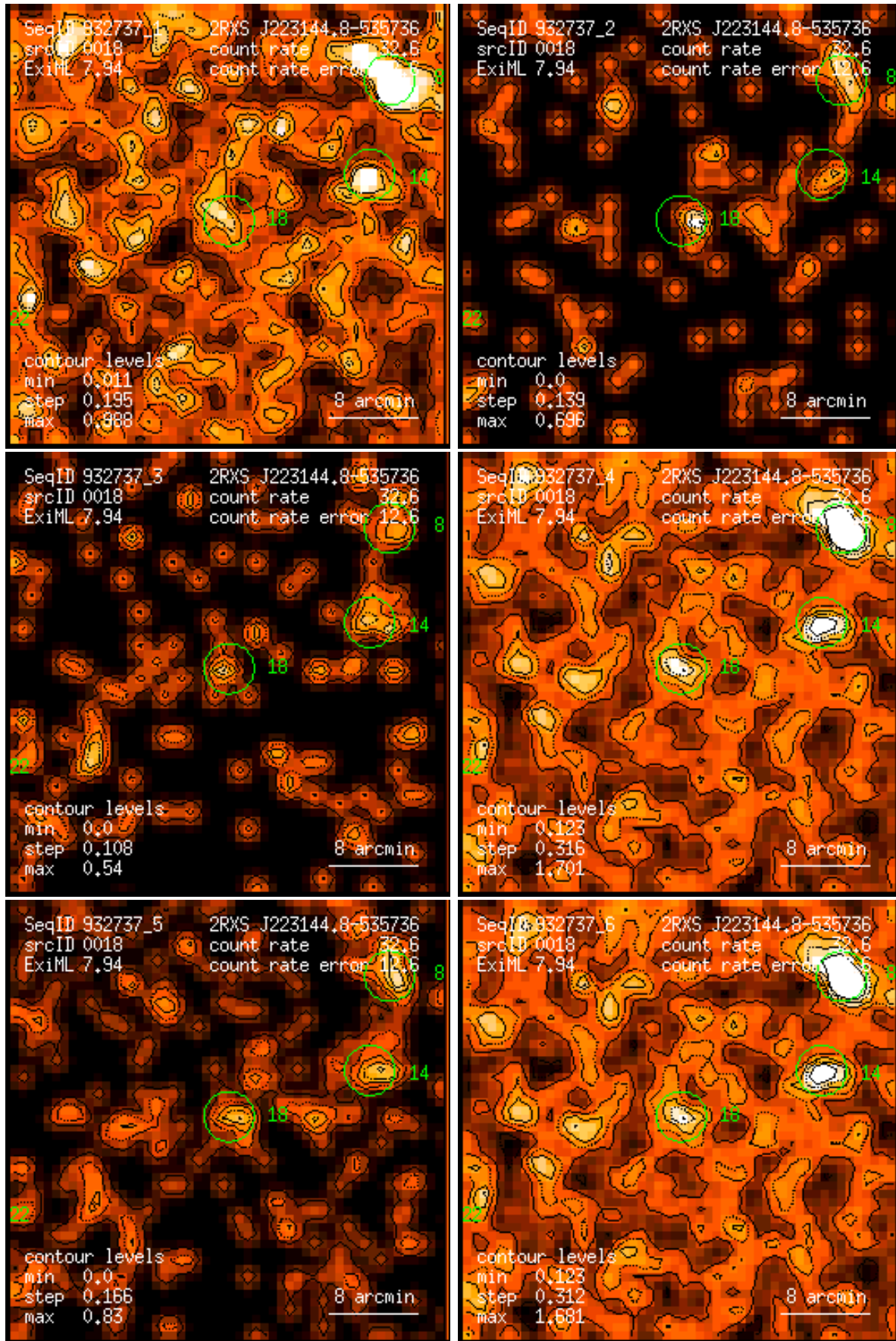
Figure 18: RASS 932737: detection 0018: band rate images, Gaussian filter: (1) PSPC channels 11 – 41, (2) 52 – 90, (3) 91 – 201, (4) 11 – 235, (5) 52 – 201, (6) 11 – 201. Broad band rates in counts/ks. Band rate contour levels in counts/ks/arcmin 2 .
