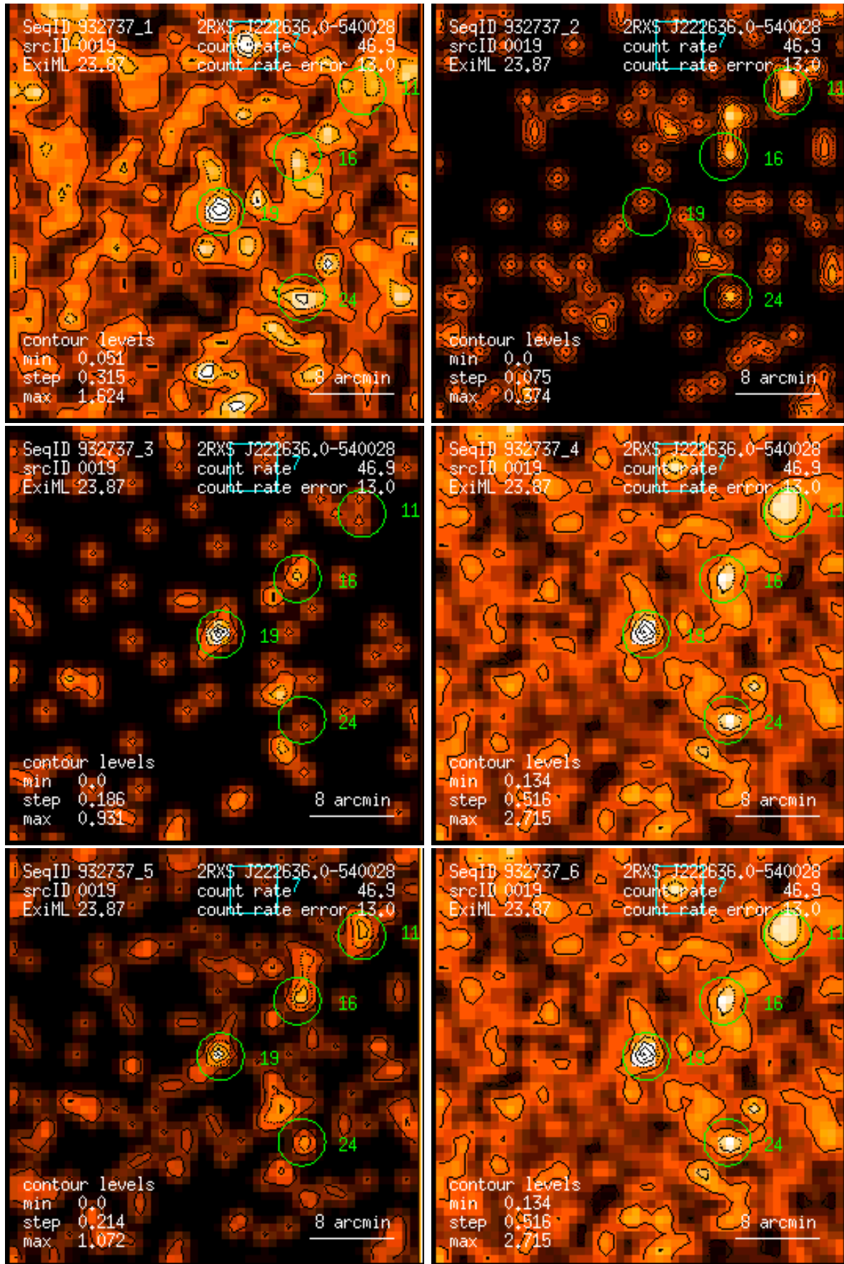
Figure 19: RASS 932737: detection 0019: band rate images, Gaussian filter: (1) PSPC channels 11 – 41, (2) 52 – 90, (3) 91 – 201, (4) 11 – 235, (5) 52 – 201, (6) 11 – 201. Broad band rates in counts/ks. Band rate contour levels in counts/ks/arcmin 2 .
