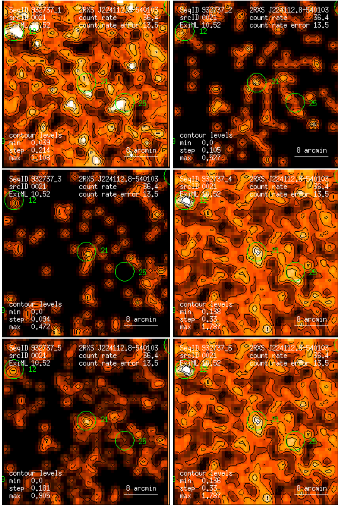
Figure 21: RASS 932737: detection 0021: band rate images, Gaussian filter: (1) PSPC channels 11 – 41, (2) 52 – 90, (3) 91 – 201, (4) 11 – 235, (5) 52 – 201, (6) 11 – 201. Broad band rates in counts/ks. Band rate contour levels in counts/ks/arcmin 2 .
