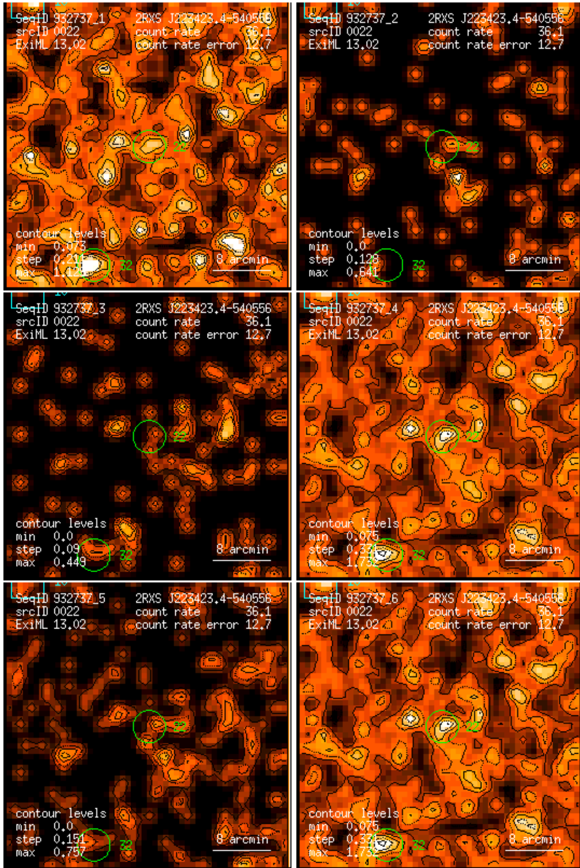
Figure 22: RASS 932737: detection 0022: band rate images, Gaussian filter: (1) PSPC channels 11 – 41, (2) 52 – 90, (3) 91 – 201, (4) 11 – 235, (5) 52 – 201, (6) 11 – 201. Broad band rates in counts/ks. Band rate contour levels in counts/ks/arcmin 2 .
