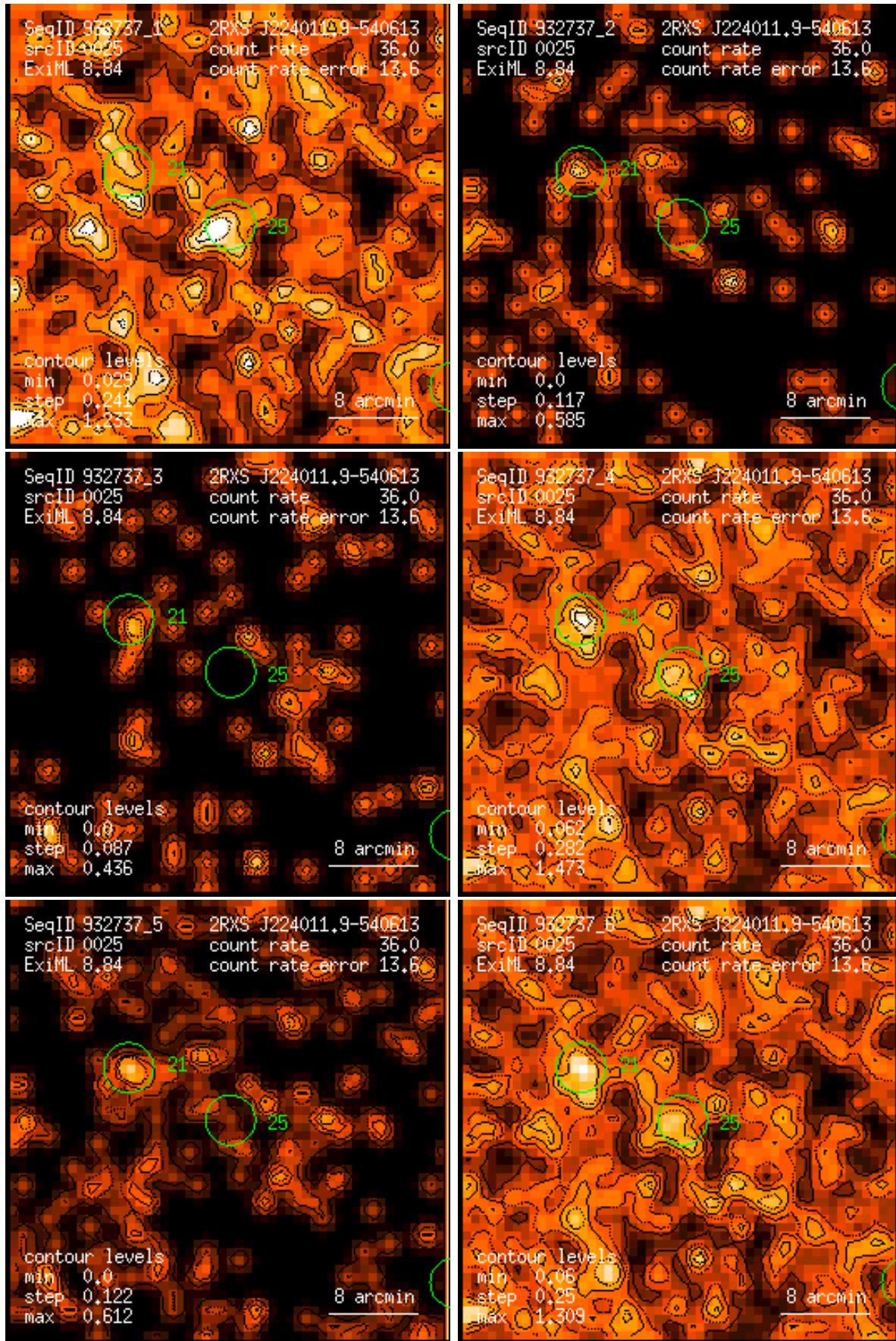
Figure 25: RASS 932737: detection 0025: band rate images, Gaussian filter: (1) PSPC channels 11 – 41, (2) 52 – 90, (3) 91 – 201, (4) 11 – 235, (5) 52 – 201, (6) 11 – 201. Broad band rates in counts/ks. Band rate contour levels in counts/ks/arcmin 2 .
