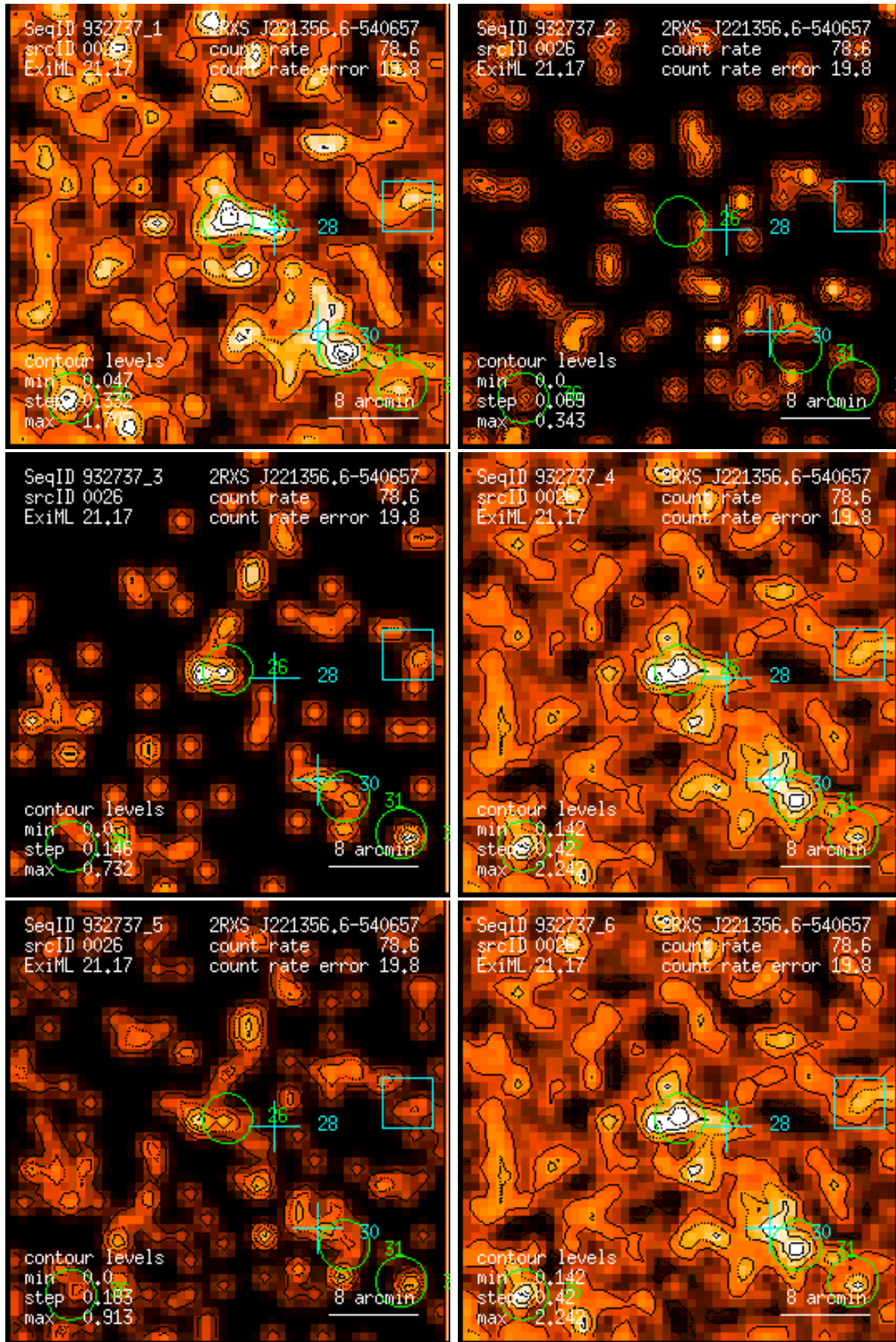
Figure 26: RASS 932737: detection 0026: band rate images, Gaussian filter: (1) PSPC channels 11 – 41, (2) 52 – 90, (3) 91 – 201, (4) 11 – 235, (5) 52 – 201, (6) 11 – 201. Broad band rates in counts/ks. Band rate contour levels in counts/ks/arcmin 2 .
