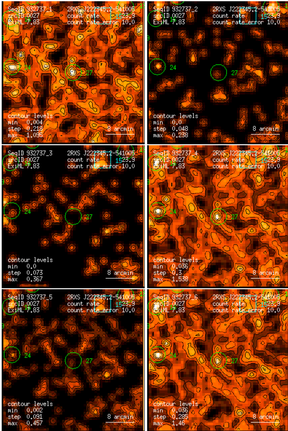
Figure 27: RASS 932737: detection 0027: band rate images, Gaussian filter: (1) PSPC channels 11 – 41, (2) 52 – 90, (3) 91 – 201, (4) 11 – 235, (5) 52 – 201, (6) 11 – 201. Broad band rates in counts/ks. Band rate contour levels in counts/ks/arcmin 2 .
