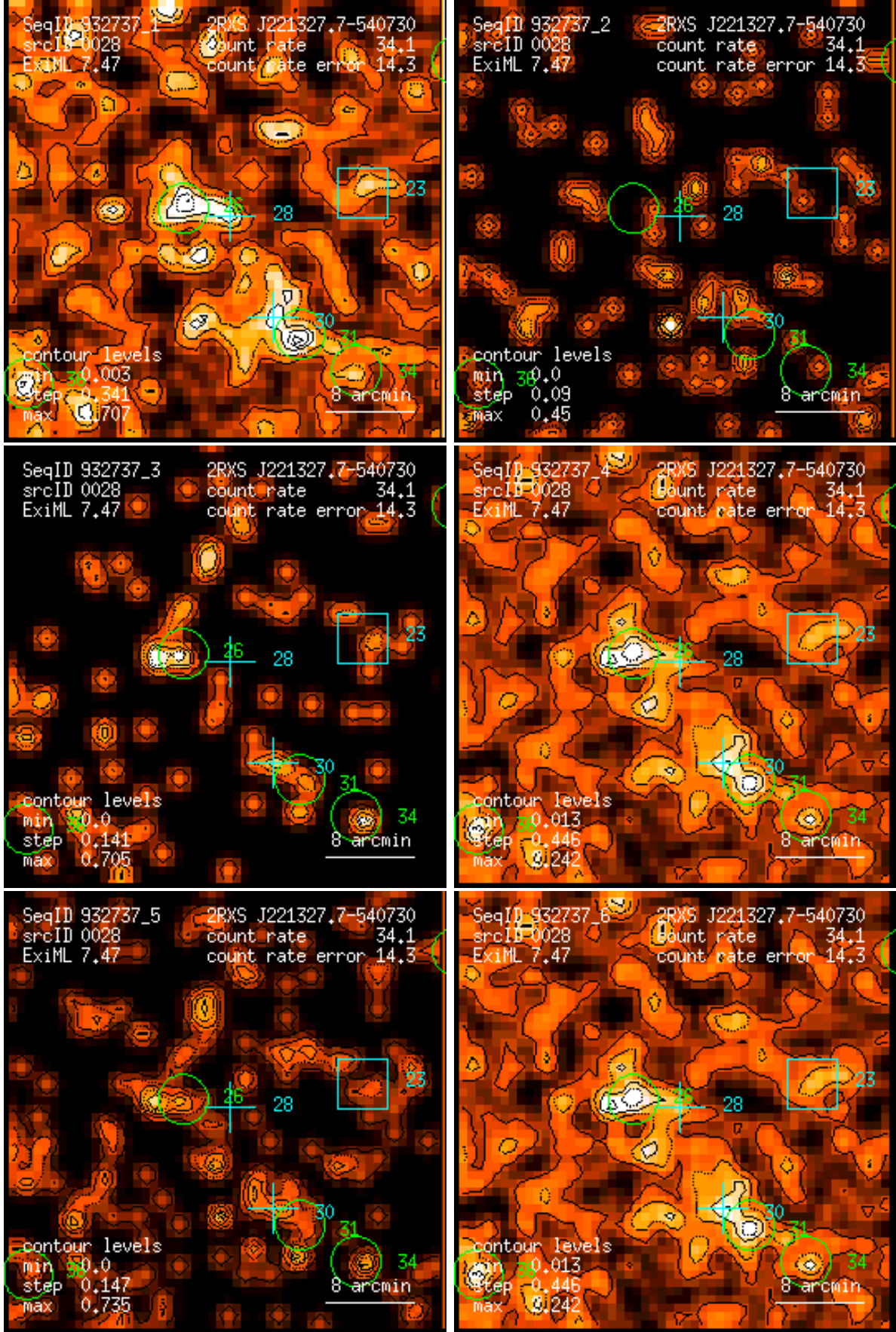
Figure 28: RASS 932737: detection 0028: band rate images, Gaussian filter: (1) PSPC channels 11 – 41, (2) 52 – 90, (3) 91 – 201, (4) 11 – 235, (5) 52 – 201, (6) 11 – 201. Broad band rates in counts/ks. Band rate contour levels in counts/ks/arcmin 2 .
