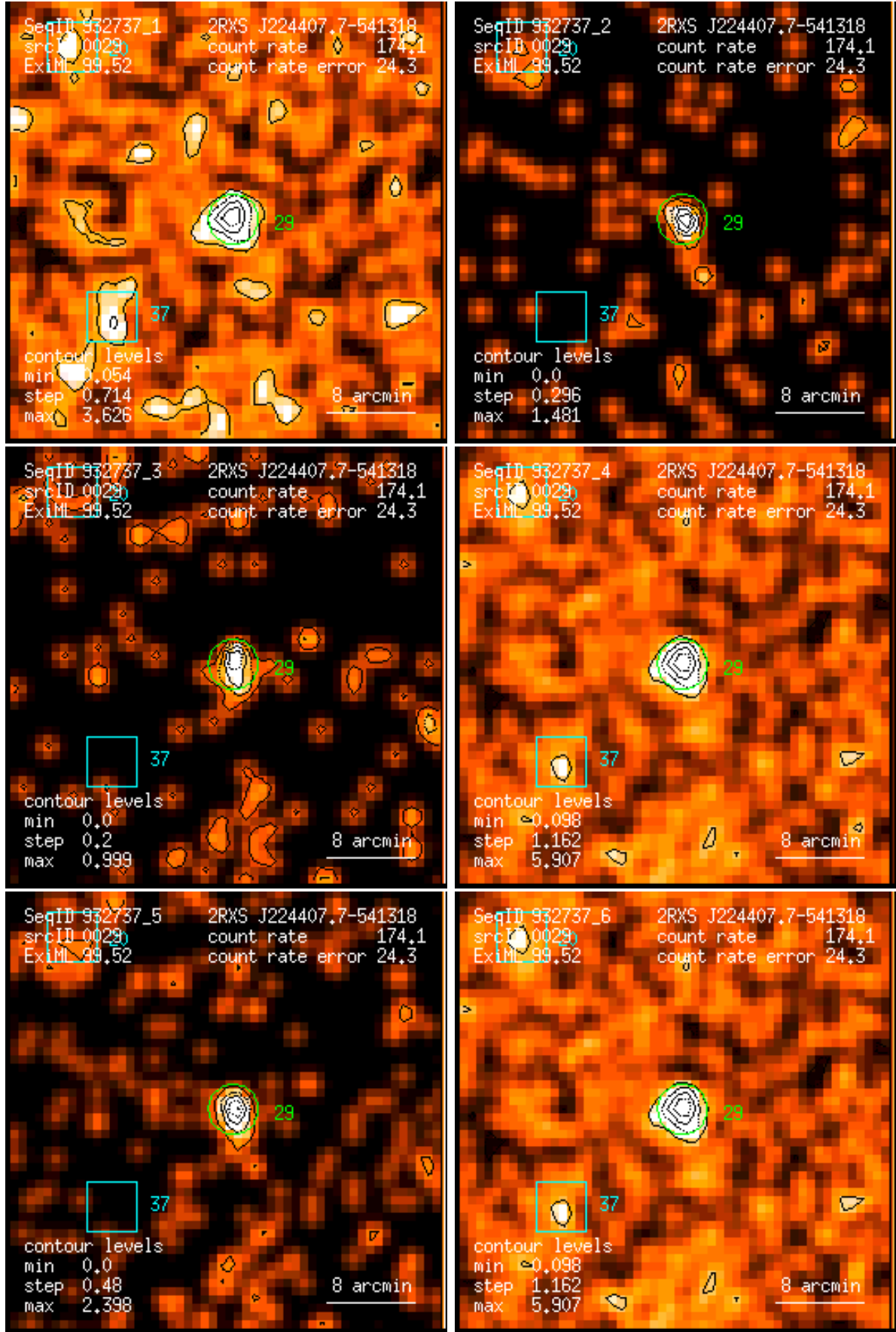
Figure 29: RASS 932737: detection 0029: band rate images, Gaussian filter: (1) PSPC channels 11 – 41, (2) 52 – 90, (3) 91 – 201, (4) 11 – 235, (5) 52 – 201, (6) 11 – 201. Broad band rates in counts/ks. Band rate contour levels in counts/ks/arcmin 2 .
