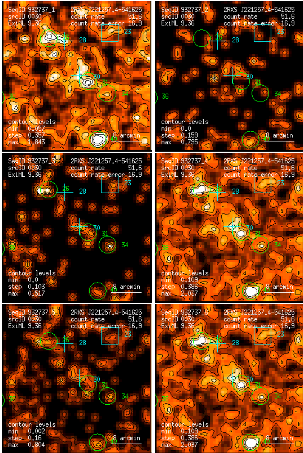
Figure 30: RASS 932737: detection 0030: band rate images, Gaussian filter: (1) PSPC channels 11 – 41, (2) 52 – 90, (3) 91 – 201, (4) 11 – 235, (5) 52 – 201, (6) 11 – 201. Broad band rates in counts/ks. Band rate contour levels in counts/ks/arcmin 2 .
