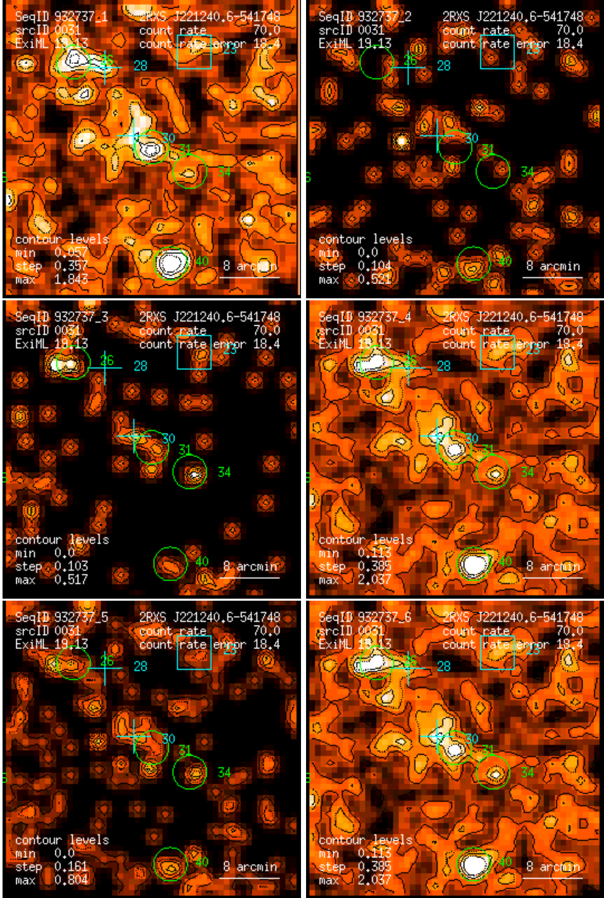
Figure 31: RASS 932737: detection 0031: band rate images, Gaussian filter: (1) PSPC channels 11 – 41, (2) 52 – 90, (3) 91 – 201, (4) 11 – 235, (5) 52 – 201, (6) 11 – 201. Broad band rates in counts/ks. Band rate contour levels in counts/ks/arcmin 2 .
