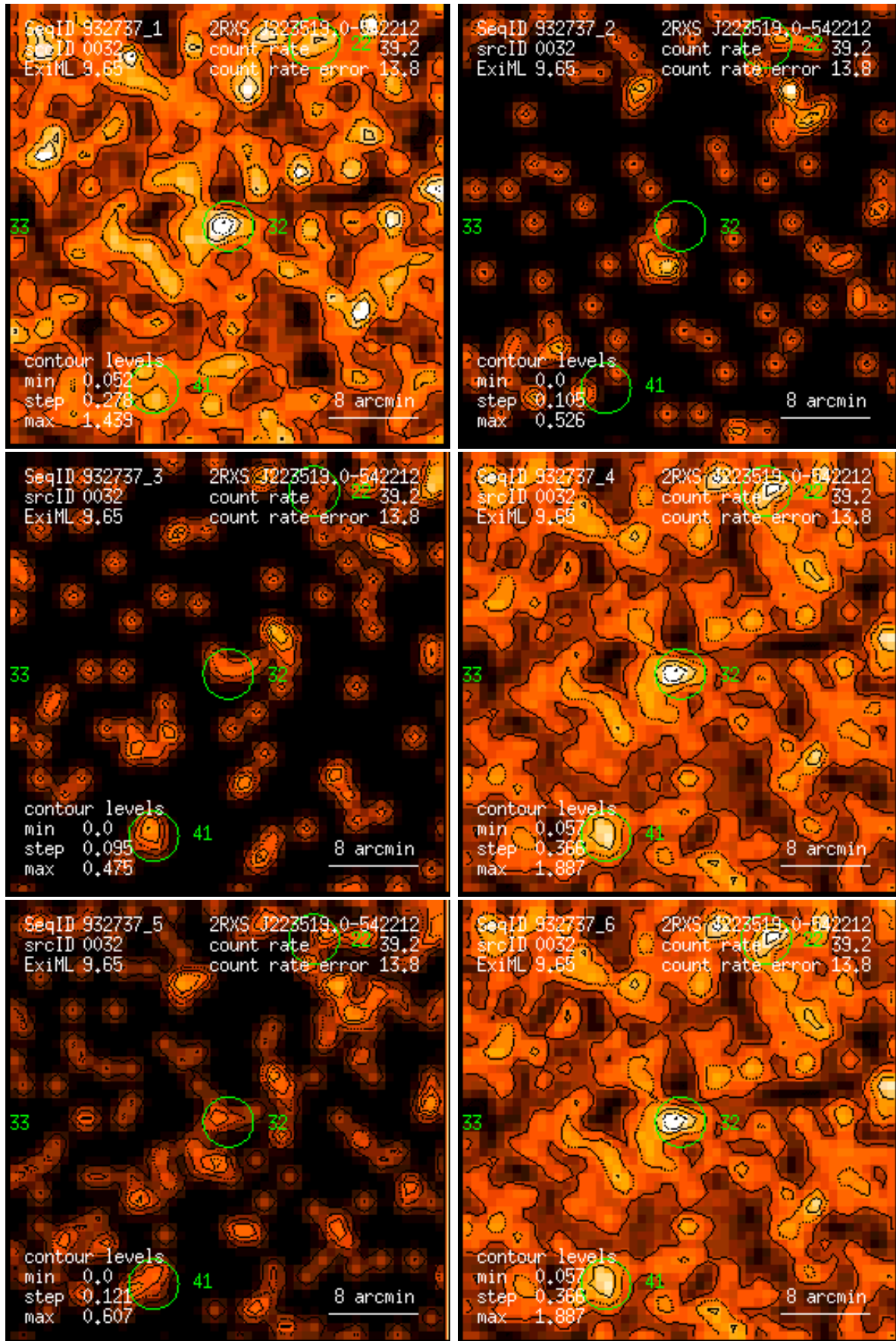
Figure 32: RASS 932737: detection 0032: band rate images, Gaussian filter: (1) PSPC channels 11 – 41, (2) 52 – 90, (3) 91 – 201, (4) 11 – 235, (5) 52 – 201, (6) 11 – 201. Broad band rates in counts/ks. Band rate contour levels in counts/ks/arcmin 2 .
