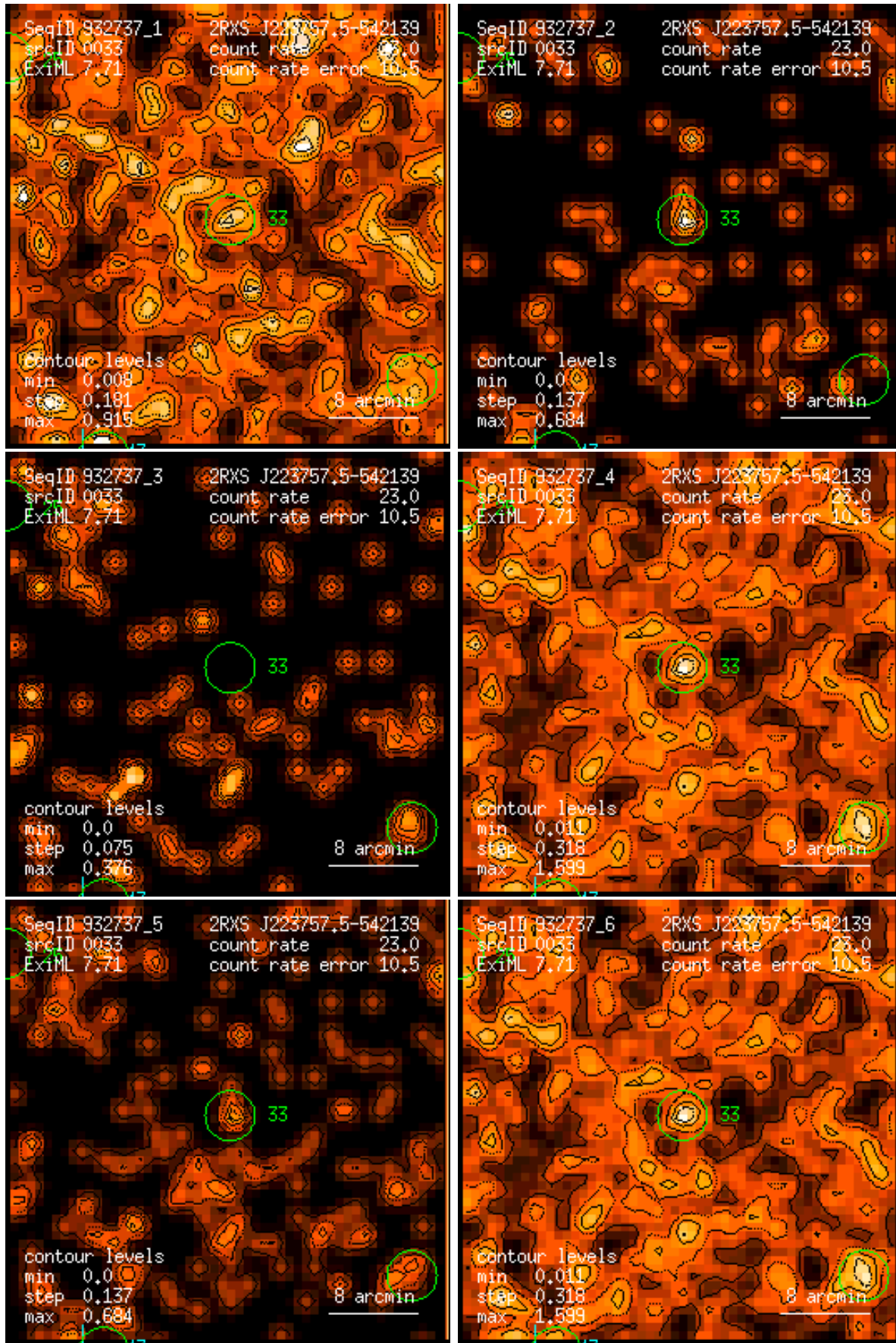
Figure 33: RASS 932737: detection 0033: band rate images, Gaussian filter: (1) PSPC channels 11 – 41, (2) 52 – 90, (3) 91 – 201, (4) 11 – 235, (5) 52 – 201, (6) 11 – 201. Broad band rates in counts/ks. Band rate contour levels in counts/ks/arcmin 2 .
