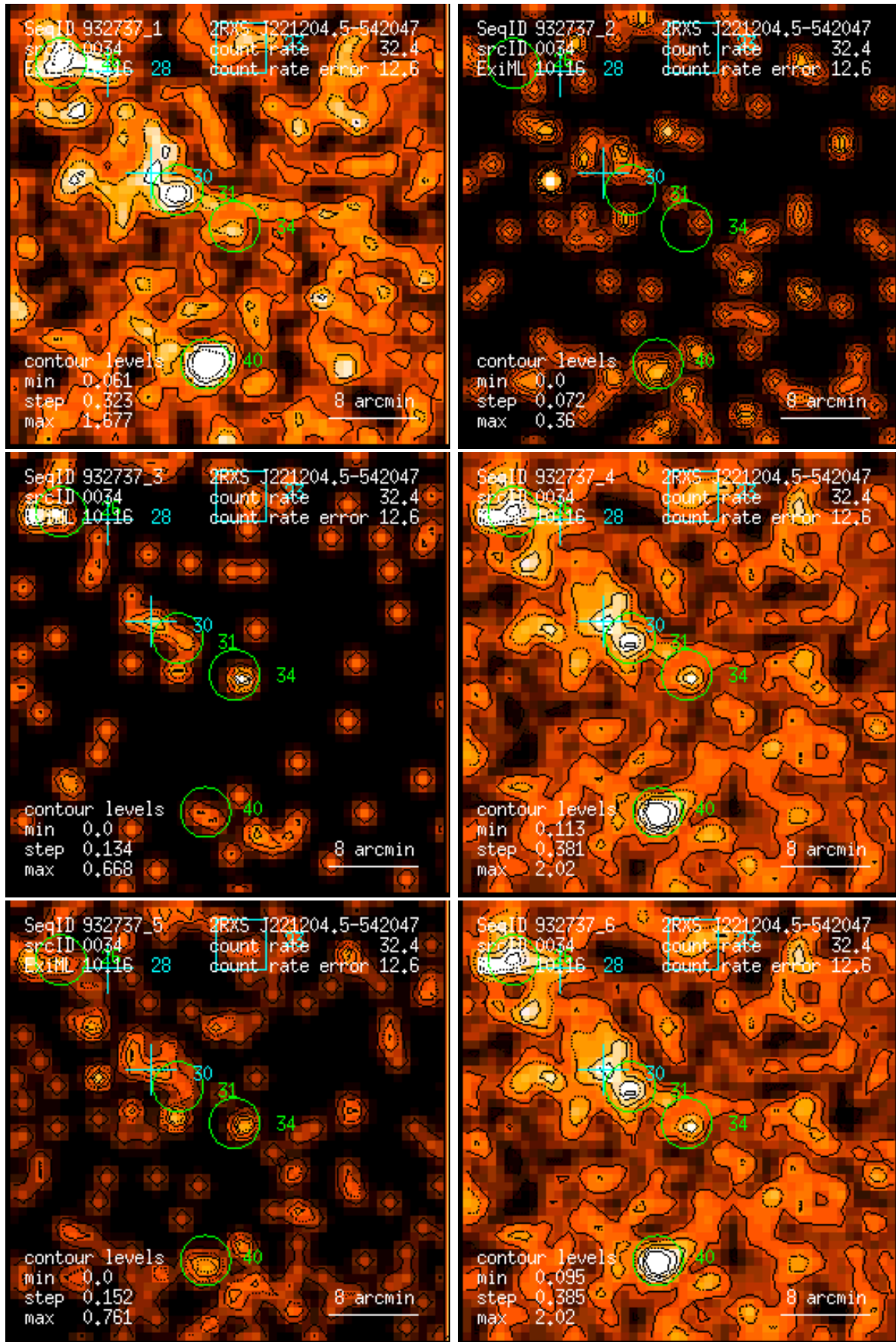
Figure 34: RASS 932737: detection 0034: band rate images, Gaussian filter: (1) PSPC channels 11 – 41, (2) 52 – 90, (3) 91 – 201, (4) 11 – 235, (5) 52 – 201, (6) 11 – 201. Broad band rates in counts/ks. Band rate contour levels in counts/ks/arcmin 2 .
