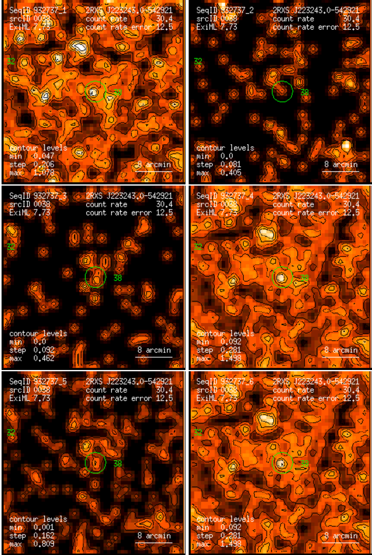
Figure 38: RASS 932737: detection 0038: band rate images, Gaussian filter: (1) PSPC channels 11 – 41, (2) 52 – 90, (3) 91 – 201, (4) 11 – 235, (5) 52 – 201, (6) 11 – 201. Broad band rates in counts/ks. Band rate contour levels in counts/ks/arcmin 2 .
