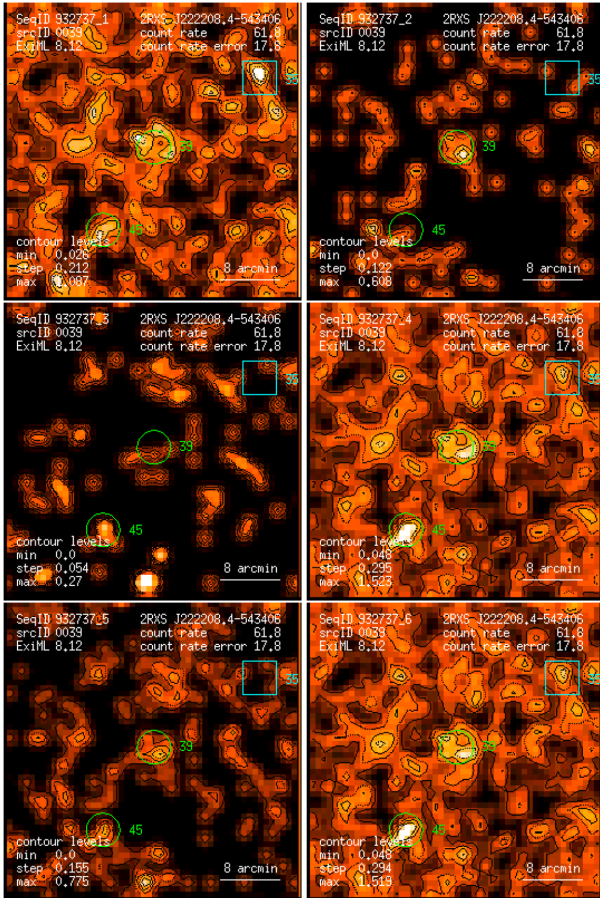
Figure 39: RASS 932737: detection 0039: band rate images, Gaussian filter: (1) PSPC channels 11 – 41, (2) 52 – 90, (3) 91 – 201, (4) 11 – 235, (5) 52 – 201, (6) 11 – 201. Broad band rates in counts/ks. Band rate contour levels in counts/ks/arcmin 2 .
