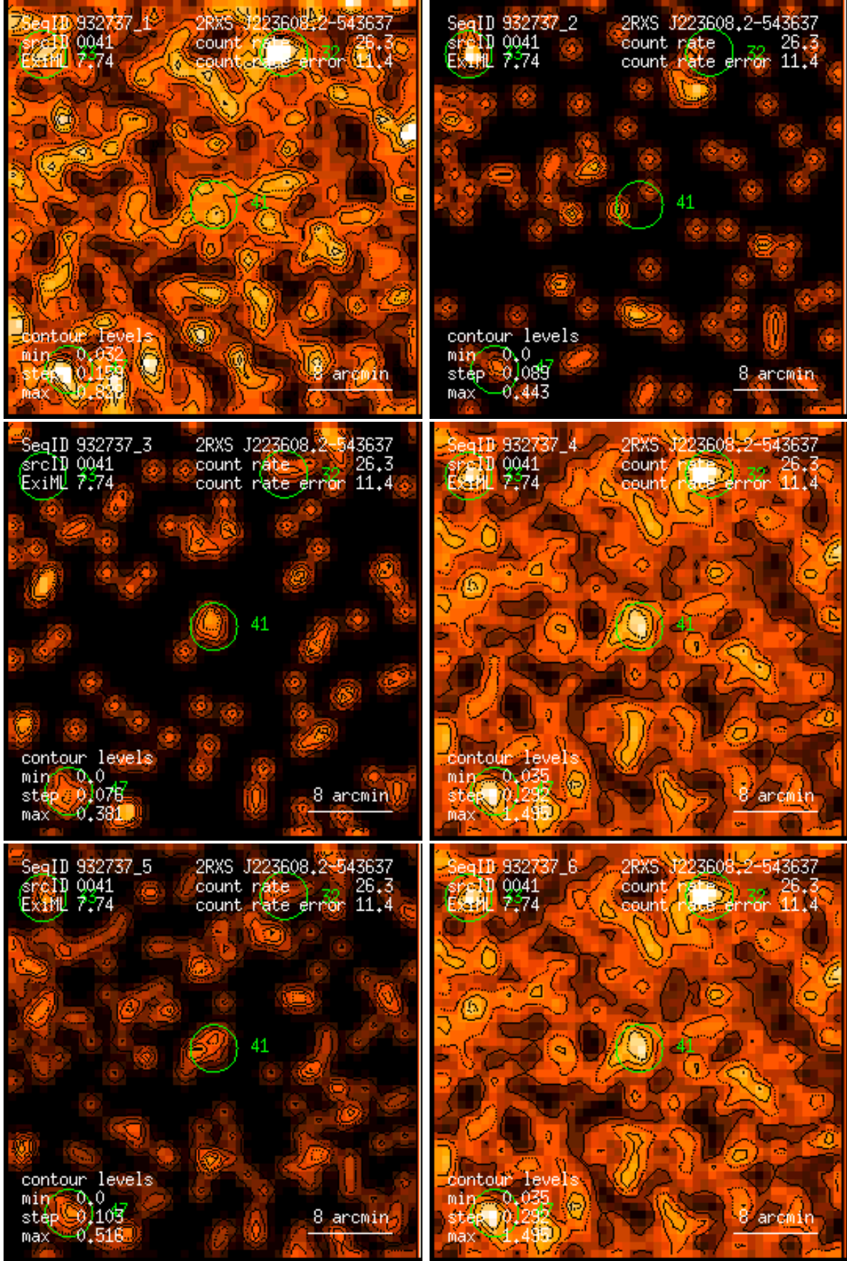
Figure 41: RASS 932737: detection 0041: band rate images, Gaussian filter: (1) PSPC channels 11 – 41, (2) 52 – 90, (3) 91 – 201, (4) 11 – 235, (5) 52 – 201, (6) 11 – 201. Broad band rates in counts/ks. Band rate contour levels in counts/ks/arcmin 2 .
